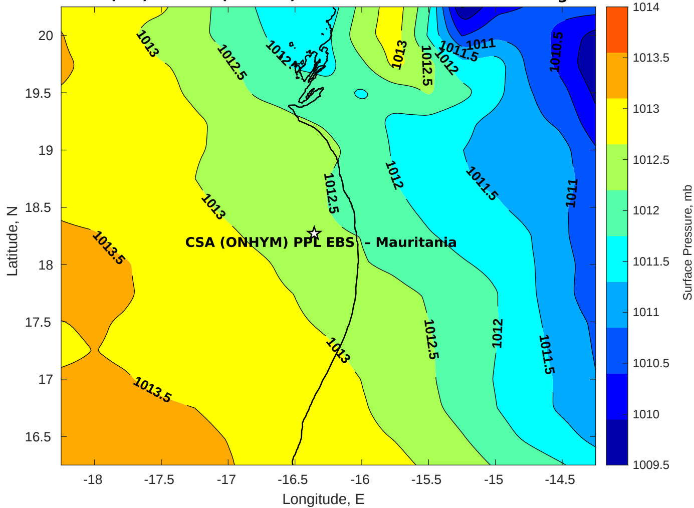
Surface Pressure (mb) for CSA (ONHYM) PPL EBS - Mauritania at 24-Aug-2025 00:00:00
