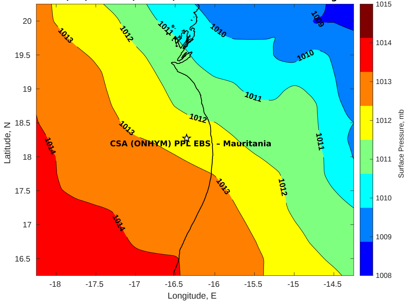
Surface Pressure (mb) for CSA (ONHYM) PPL EBS - Mauritania at 25-Aug-2025 00:00:00
