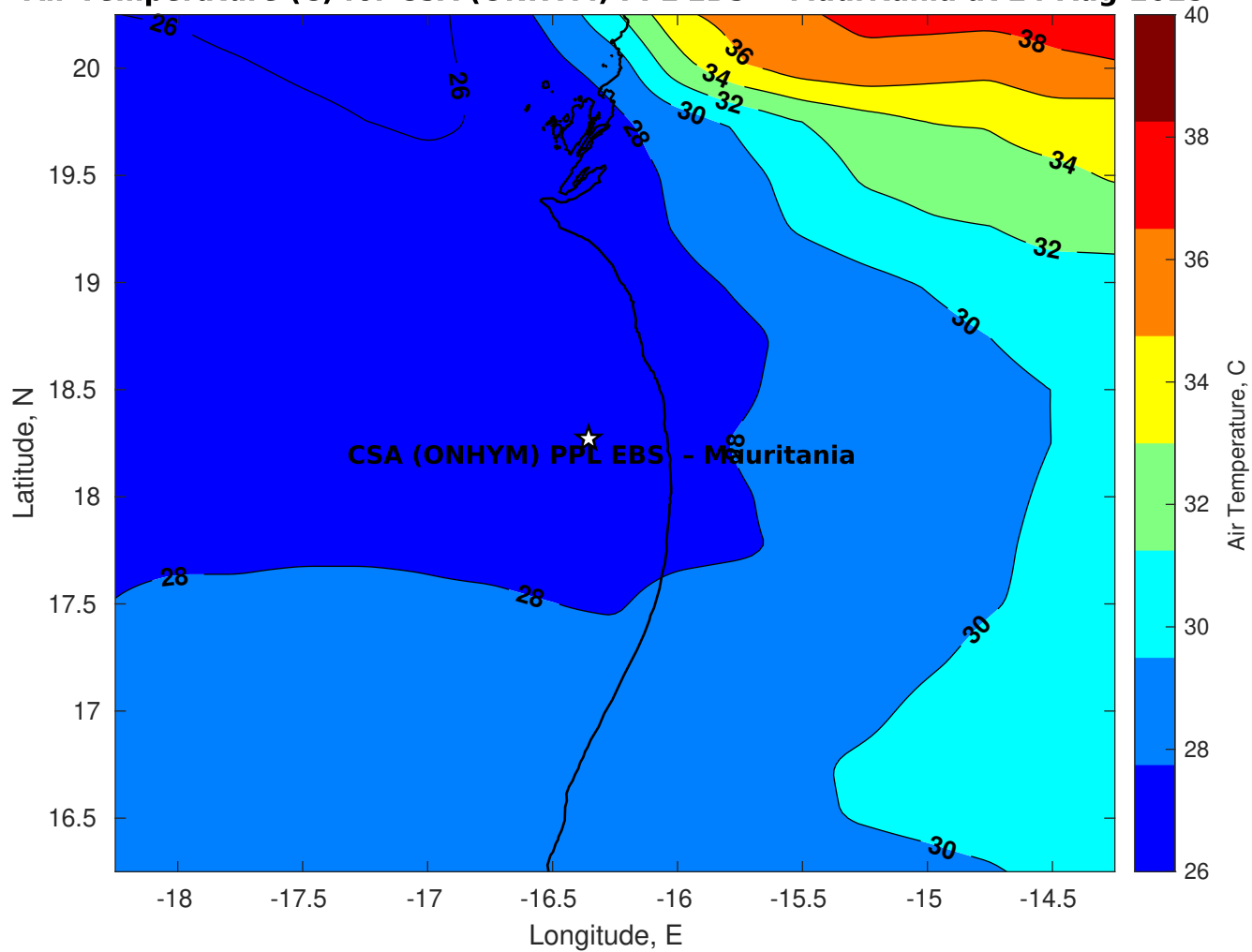
Air Temperature (C) for CSA (ONHYM) PPL EBS - Mauritania at 24-Aug-2025
