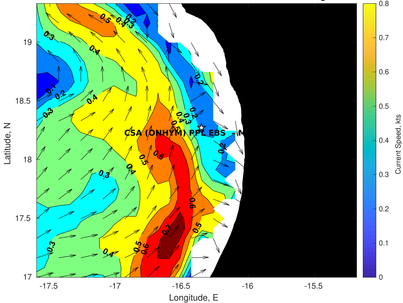
Surface Currents for CSA (ONHYM) PPL EBS - Mauritania at 23-Aug-2025 00:00:00
