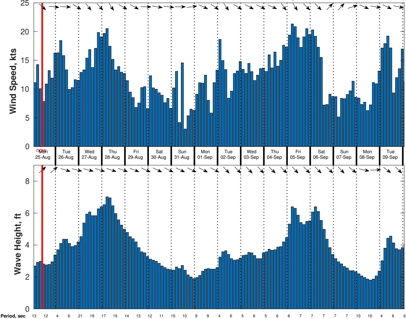
Wind & Wave Forecast for CSA (ONHYM) PPL EBS - Mauritania from 24-Aug-2025 01:00:00 to 09-Sep-2025 01:00:00
