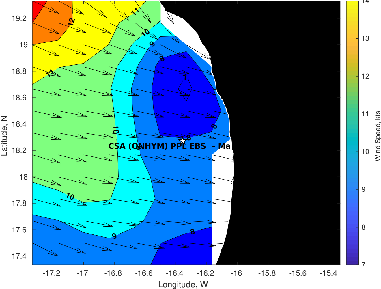
Winds (kts) for CSA (ONHYM) PPL EBS - Mauritania at 24-Aug-2025 09:00:00
