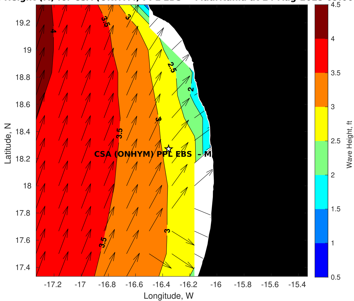
Wave Height (ft) for CSA (ONHYM) PPL EBS - Mauritania at 24-Aug-2025 09:00:00
