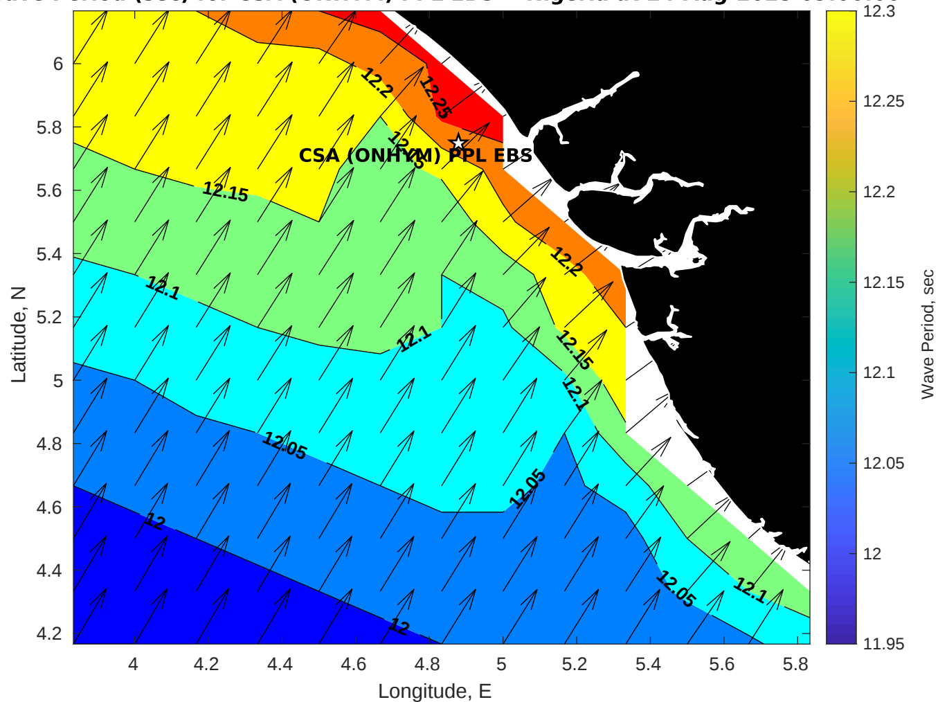
Wave Period (sec) for CSA (ONHYM) PPL EBS - Nigeria at 24-Aug-2025 09:00:00
