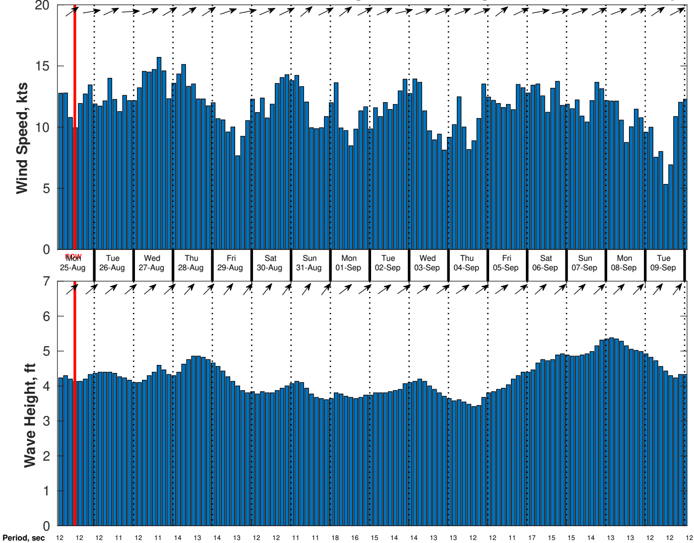
Wind & Wave Forecast for CSA (ONHYM) PPL EBS - Nigeria from 24-Aug-2025 02:00:00 to 09-Sep-2025 02:00:00
