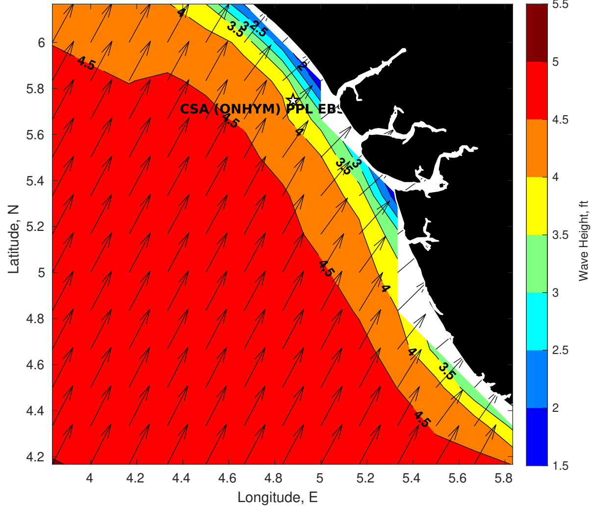
Wave Height (ft) for CSA (ONHYM) PPL EBS - Nigeria at 24-Aug-2025 09:00:00
