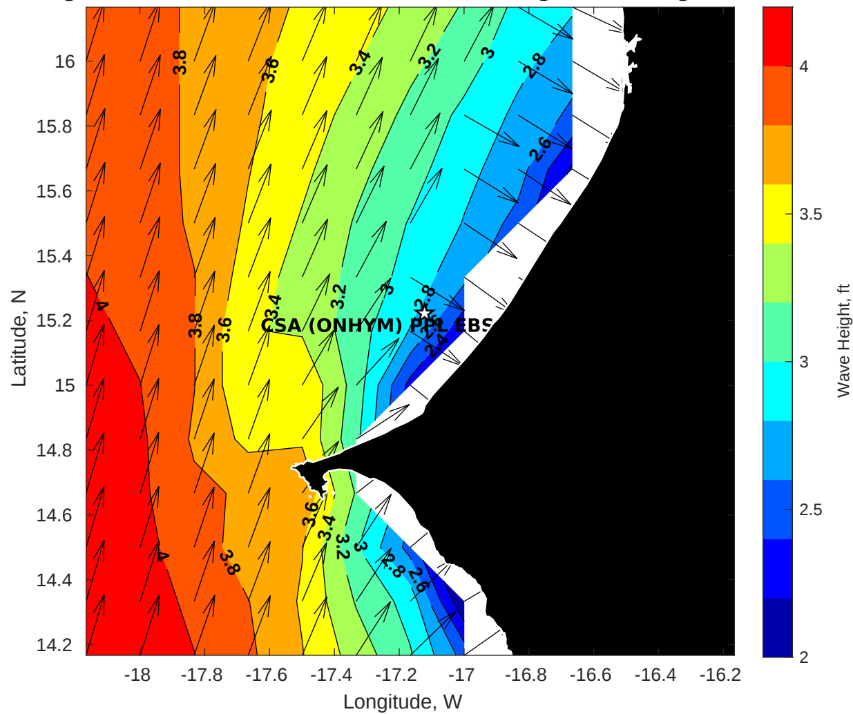
Wave Height (ft) for CSA (ONHYM) PPL EBS - Senegal at 24-Aug-2025 09:00:00
