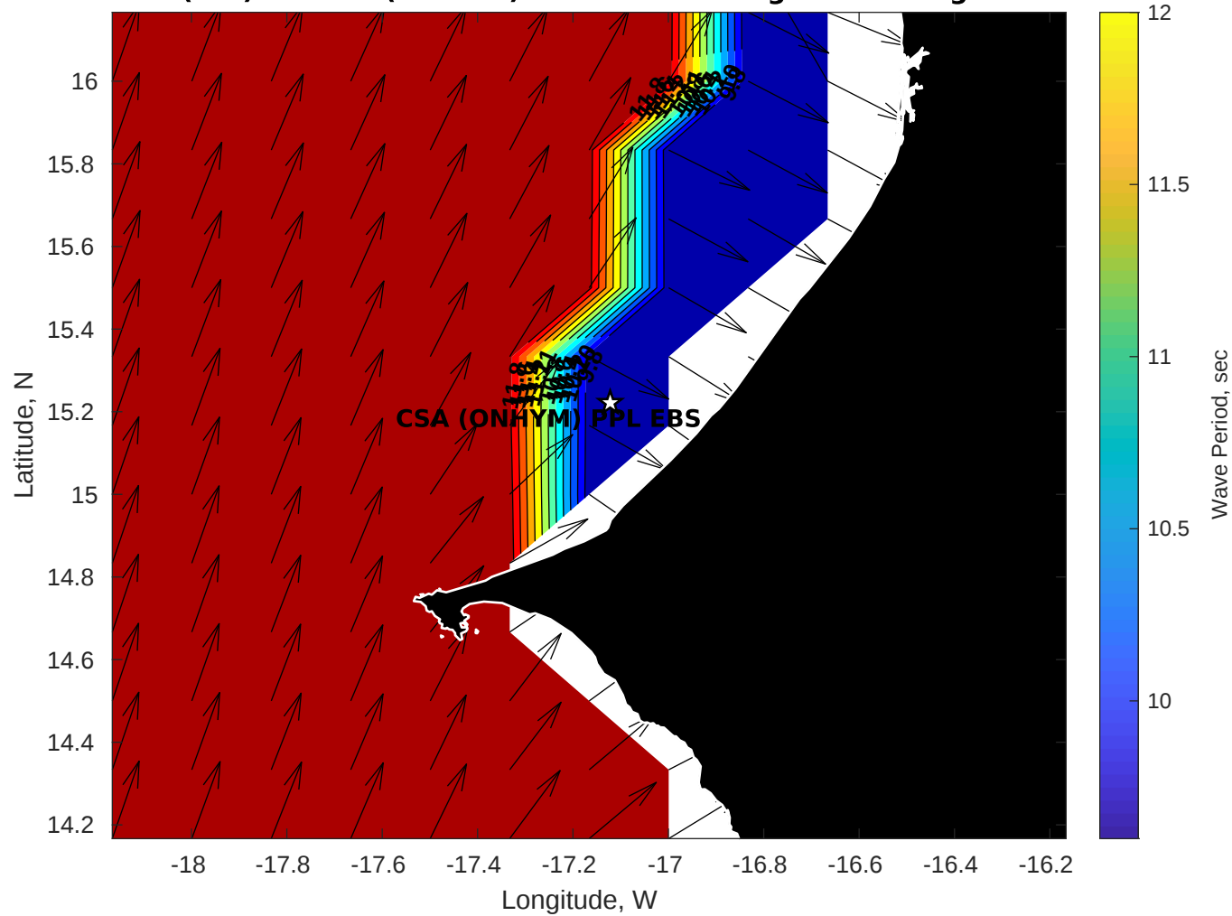
Wave Period (sec) for CSA (ONHYM) PPL EBS - Senegal at 24-Aug-2025 09:00:00
