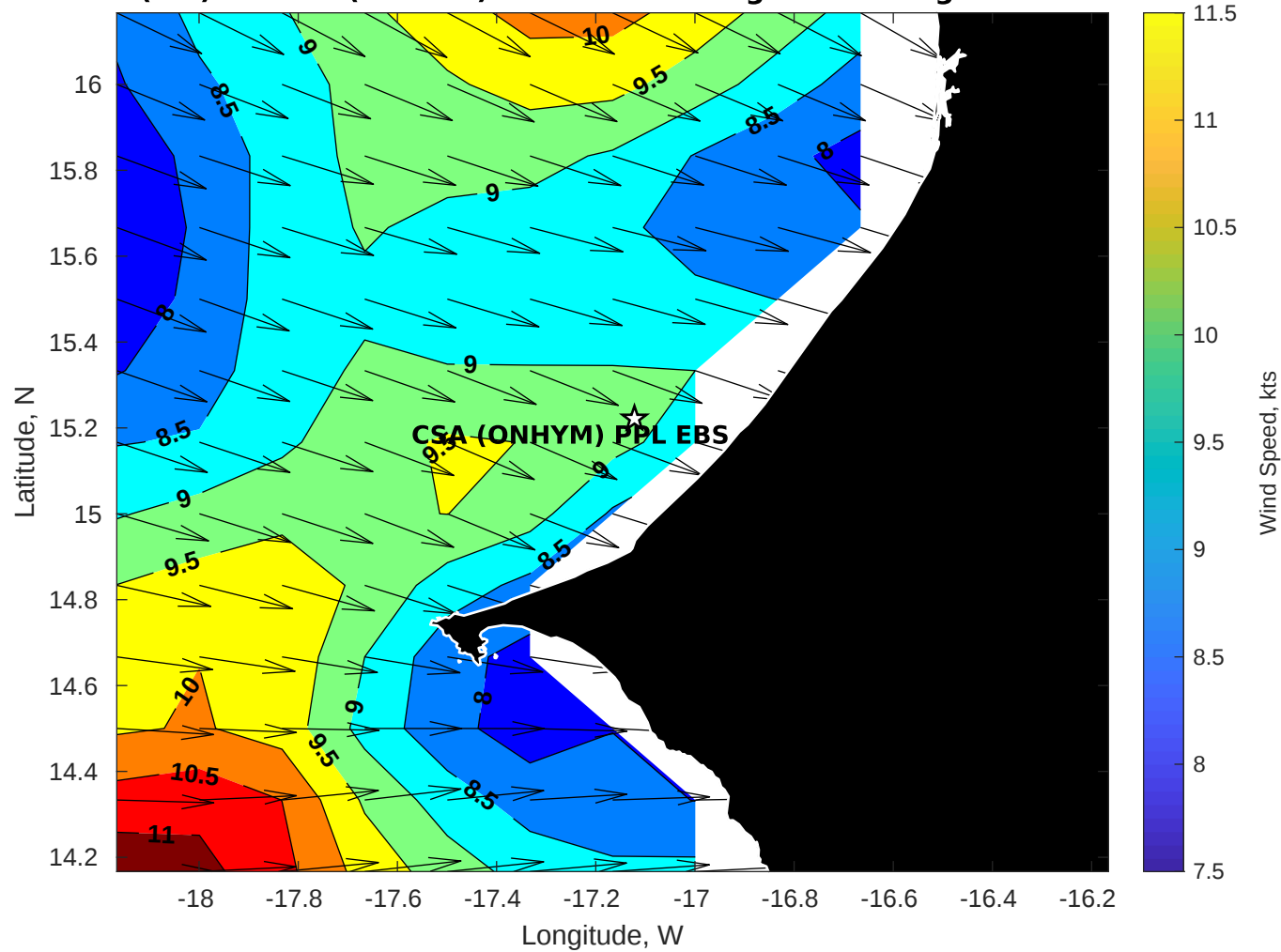
Winds (kts) for CSA (ONHYM) PPL EBS - Senegal at 24-Aug-2025 09:00:00
