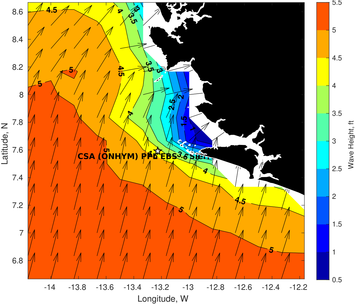
Wave Height (ft) for CSA (ONHYM) PPL EBS - Sierra Leone at 24-Aug-2025 09:00:00
