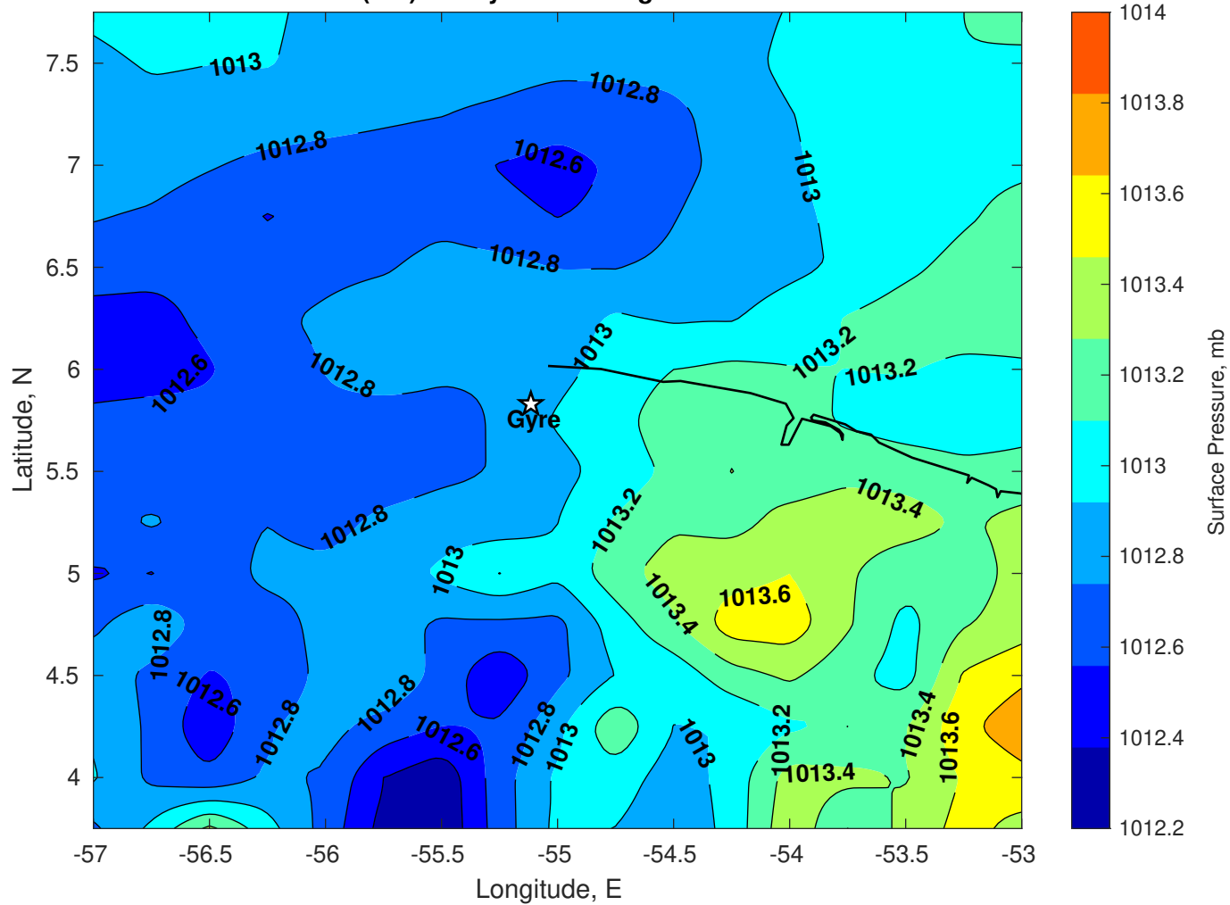
Surface Pressure (mb) for Gyre at 24-Aug-2025 00:00:00
