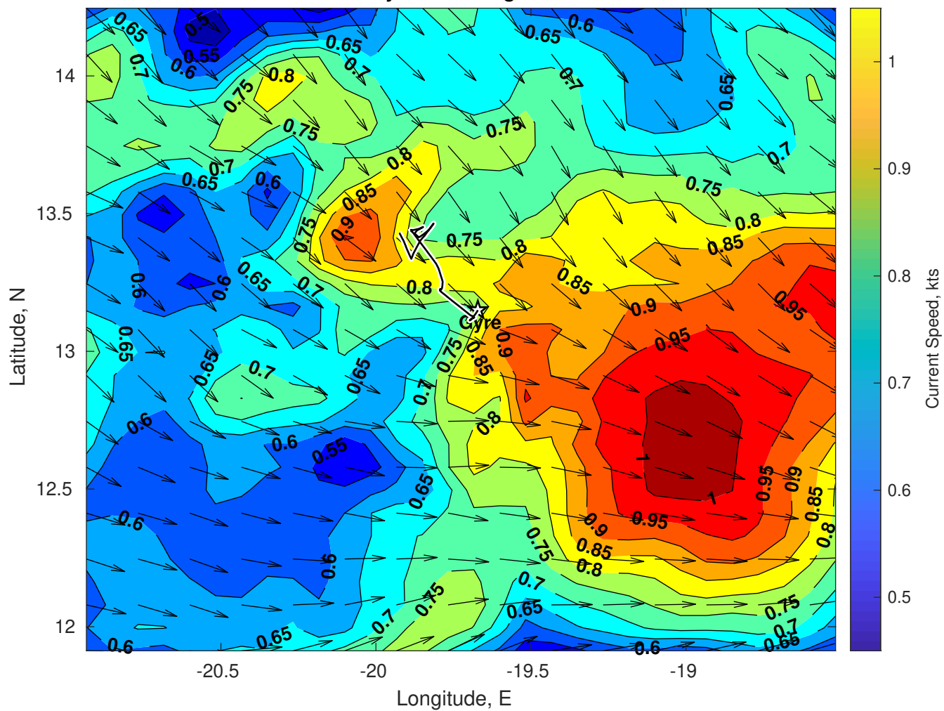
Surface Currents for Gyre at 23-Aug-2025 00:00:00
