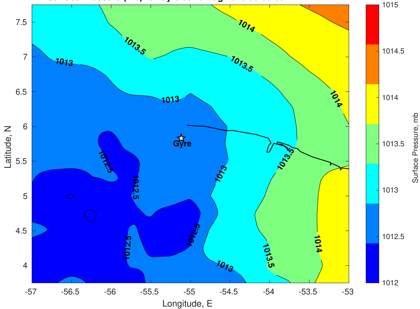
Surface Pressure (mb) for Gyre at 26-Aug-2025 00:00:00
