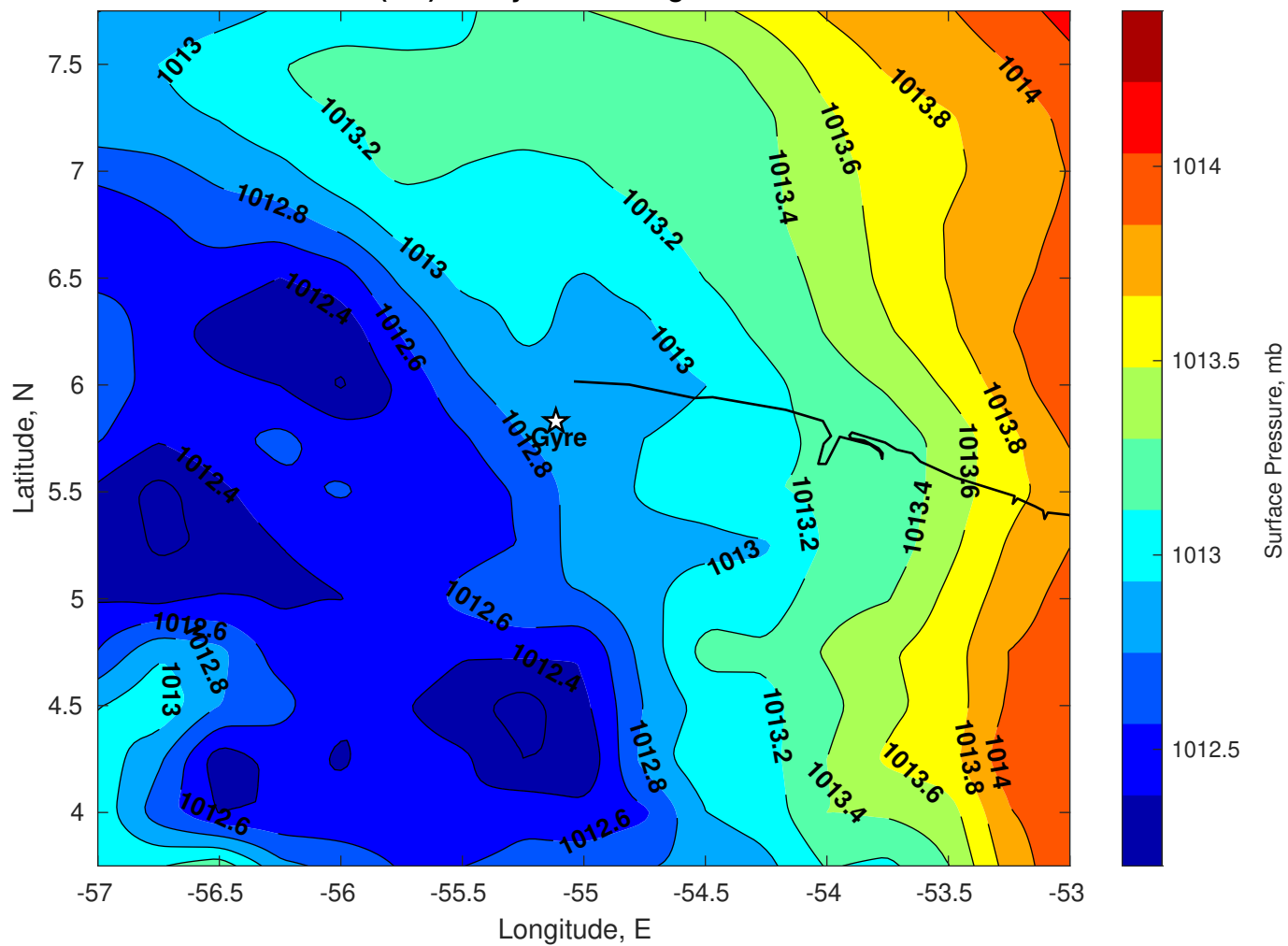
Surface Pressure (mb) for Gyre at 25-Aug-2025 00:00:00
