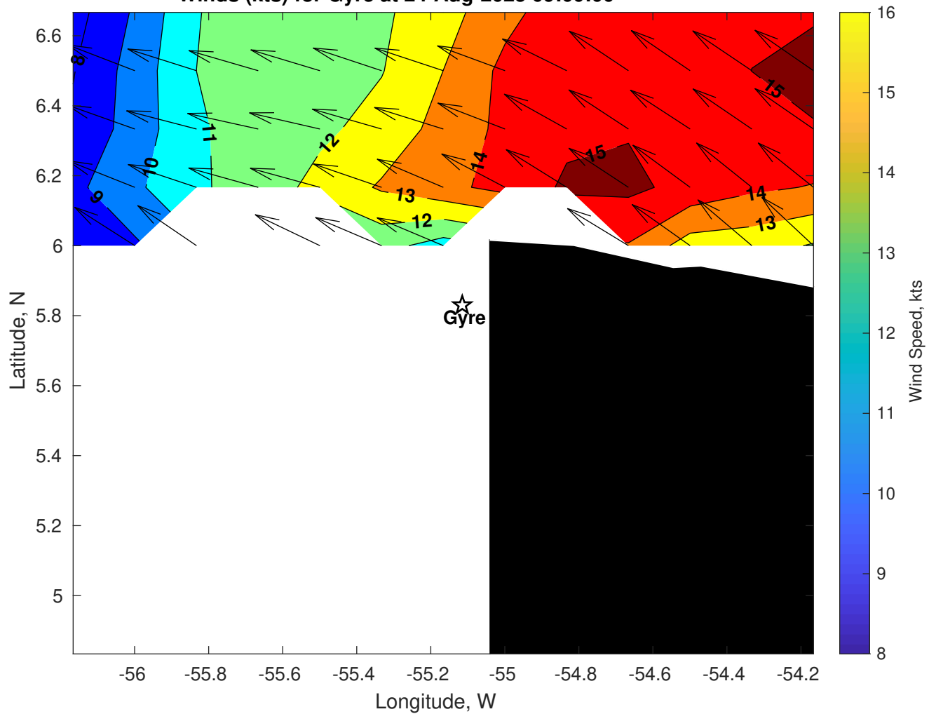
Winds (kts) for Gyre at 24-Aug-2025 09:00:00
