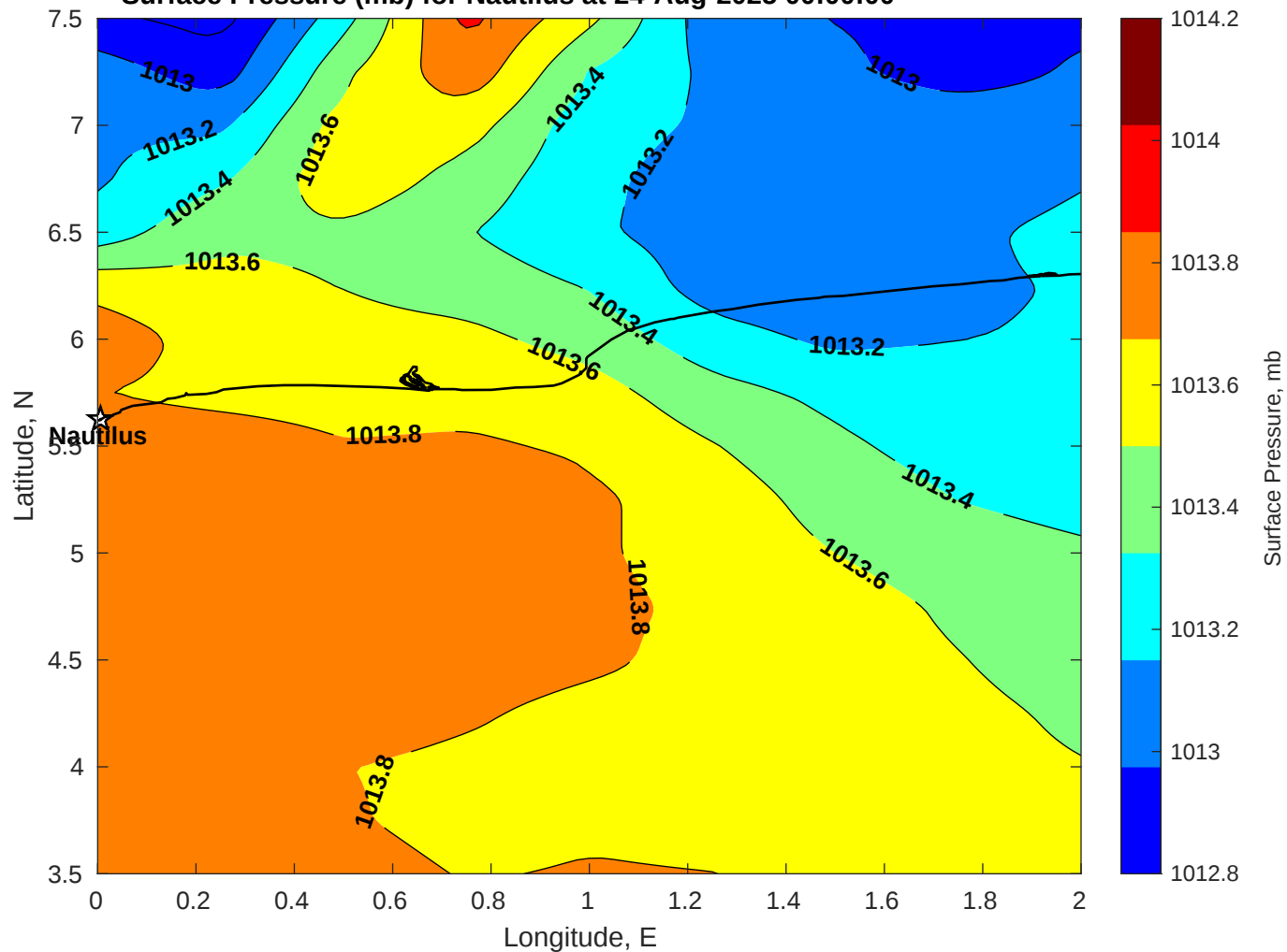
Surface Pressure (mb) for Nautilus at 24-Aug-2025 00:00:00
