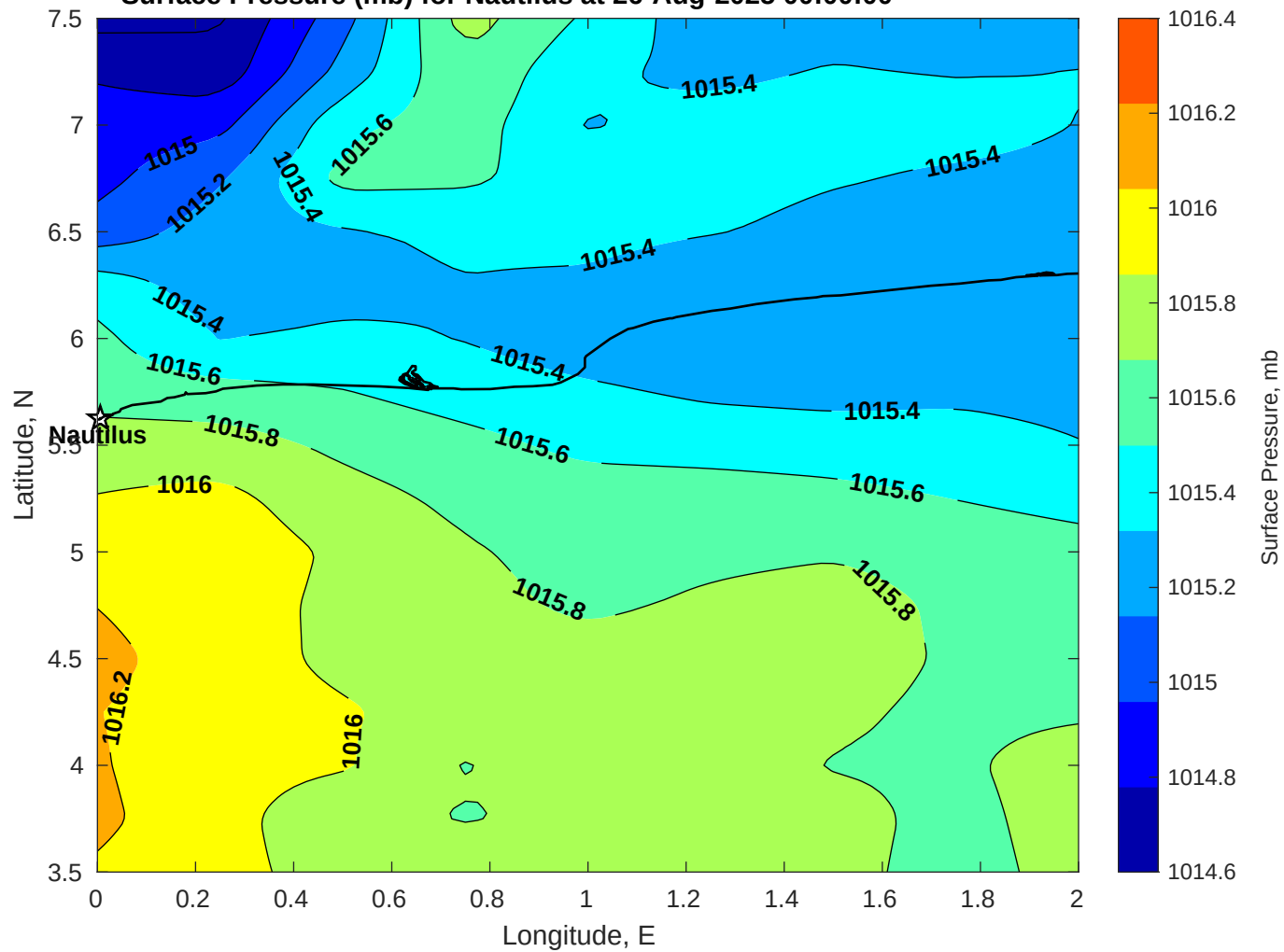
Surface Pressure (mb) for Nautilus at 26-Aug-2025 00:00:00
