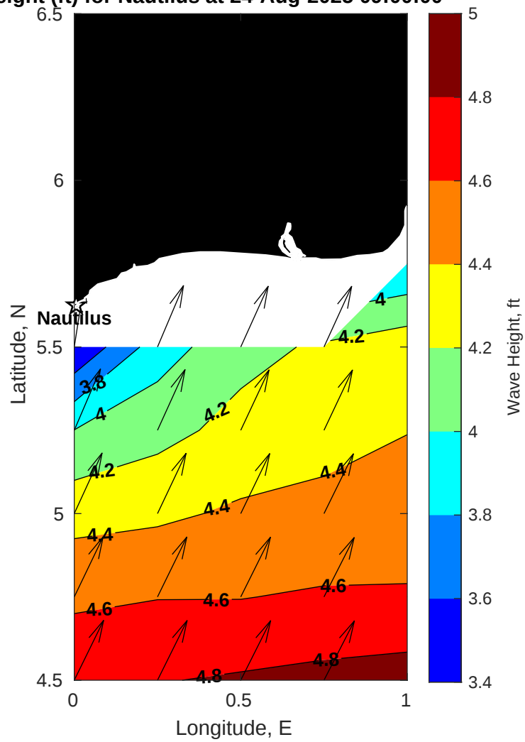
Wave Height (ft) for Nautilus at 24-Aug-2025 09:00:00
