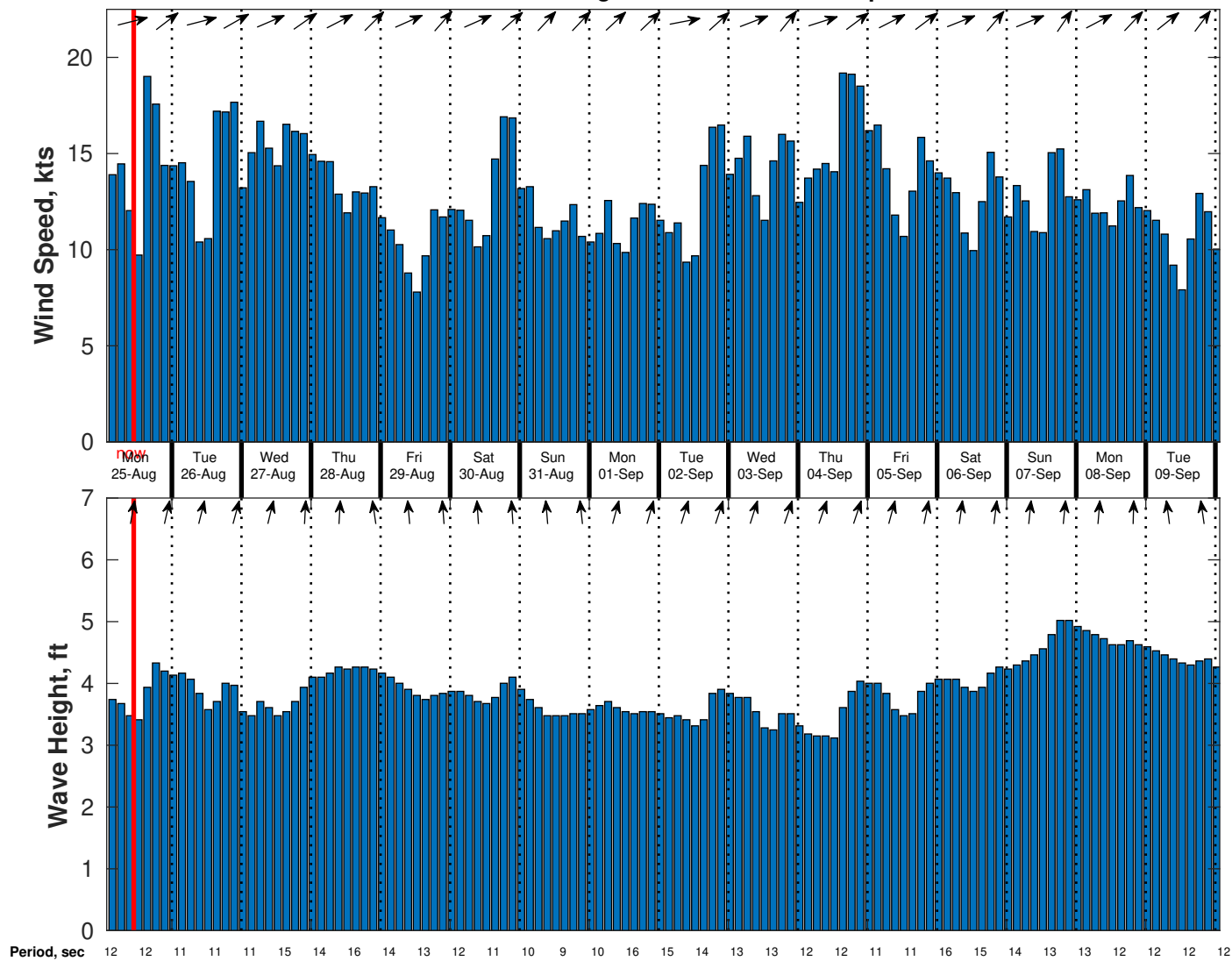
Wind & Wave Forecast for Nautilus from 24-Aug-2025 02:00:00 to 09-Sep-2025 02:00:00
