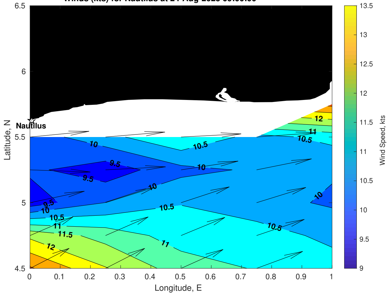
Winds (kts) for Nautilus at 24-Aug-2025 09:00:00
