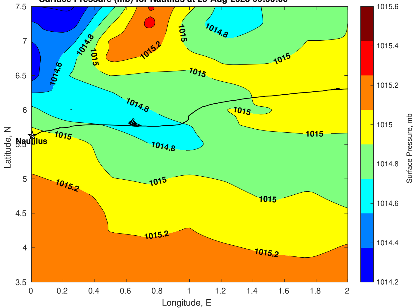
Surface Pressure (mb) for Nautilus at 25-Aug-2025 00:00:00
