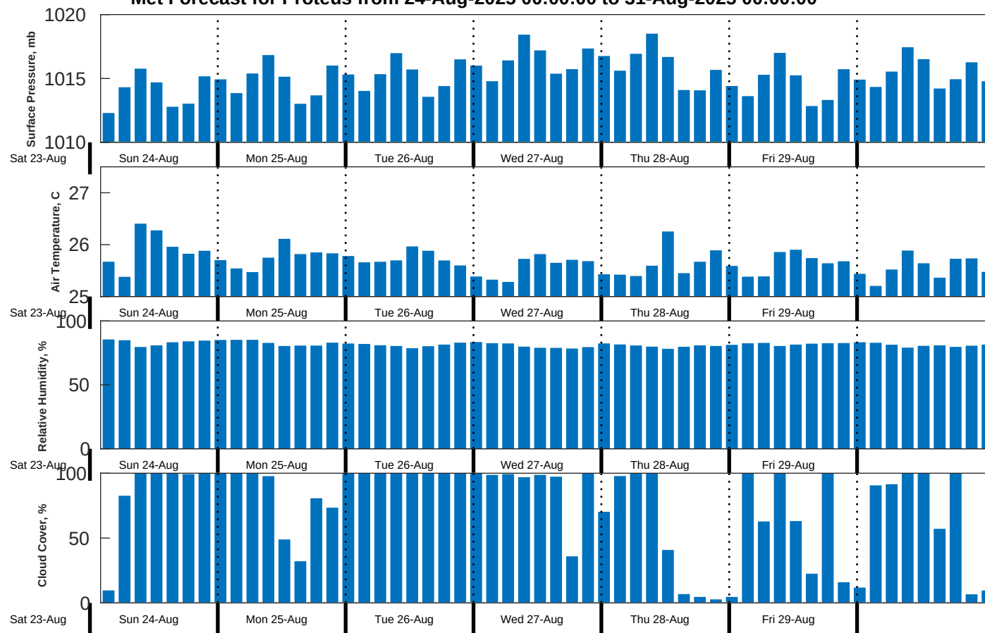
Met Forecast for Proteus from 24-Aug-2025 00:00:00 to 31-Aug-2025 00:00:00
