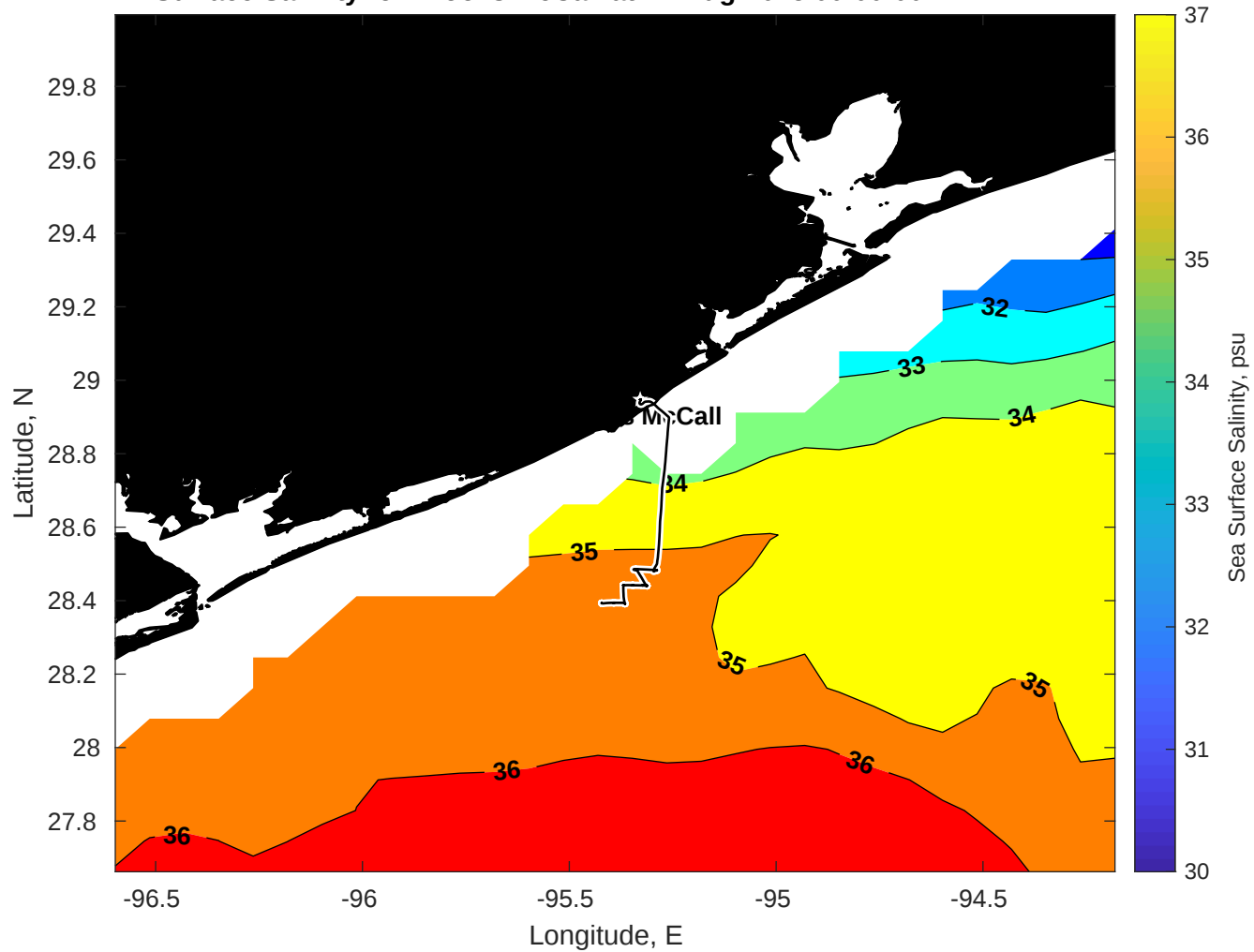
Surface Salinity for Brooks McCall at 24-Aug-2025 00:00:00
