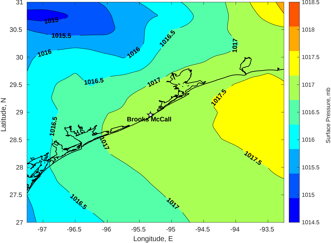
Surface Pressure (mb) for Brooks McCall at 27-Aug-2025 00:00:00
