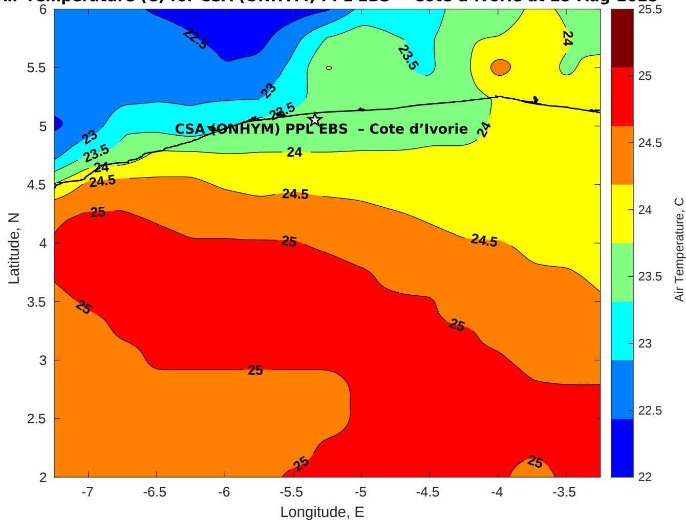
Air Temperature (C) for CSA (ONHYM) PPL EBS - Cote d'Ivoire at 25-Aug-2025
