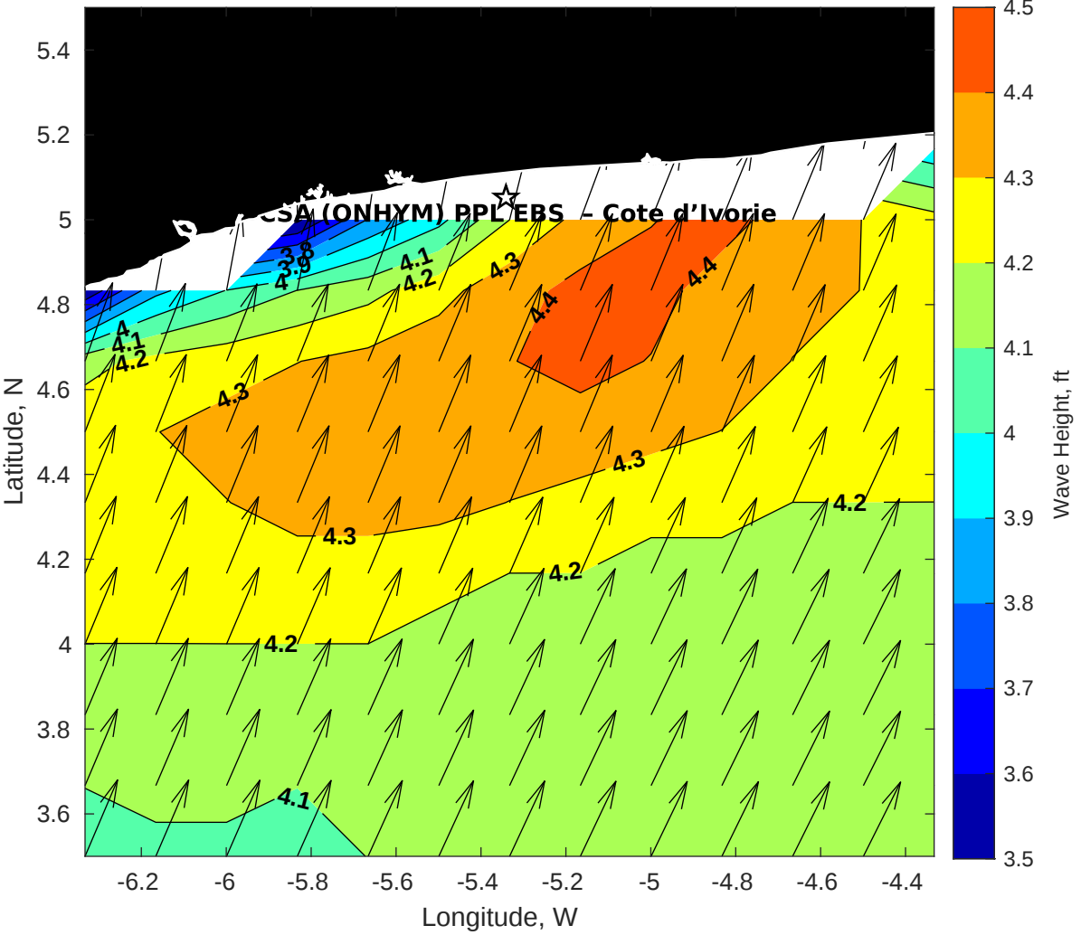
Wave Height (ft) for CSA (ONHYM) PPL EBS - Cote d'Ivoire at 25-Aug-2025 09:00:00
