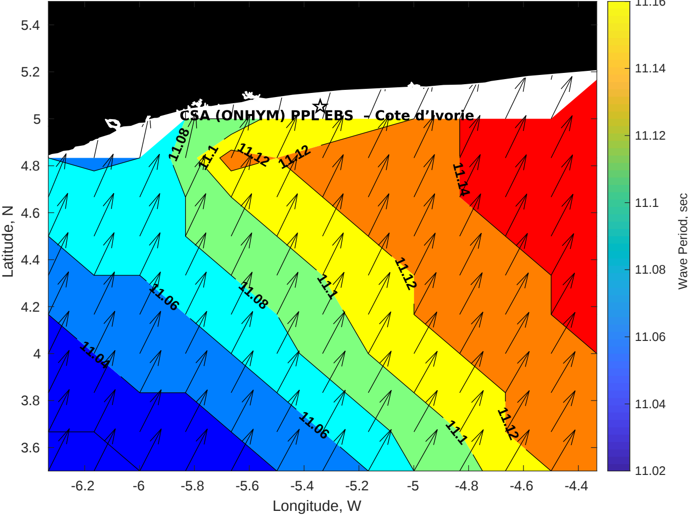
Wave Period (sec) for CSA (ONHYM) PPL EBS - Cote d'Ivoire at 25-Aug-2025 09:00:00
