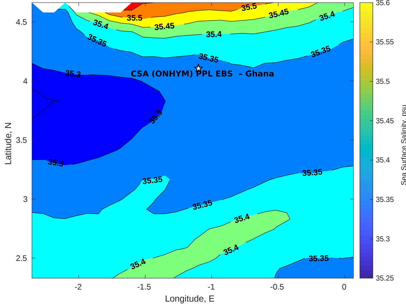
Surface Salinity for CSA (ONHYM) PPL EBS - Ghana at 24-Aug-2025 00:00:00
