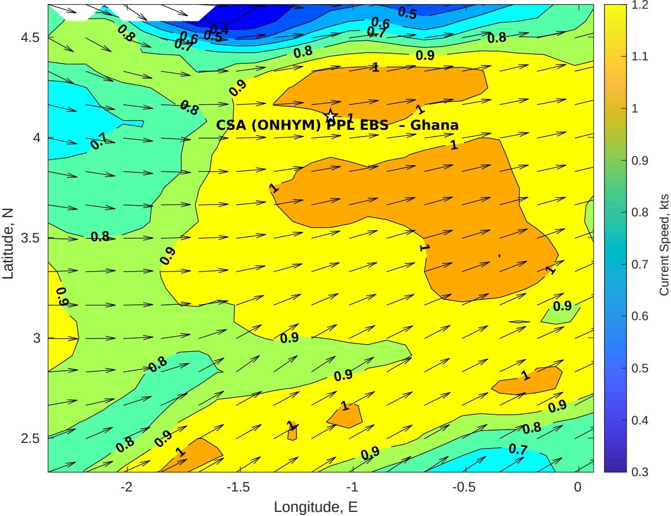
Surface Currents for CSA (ONHYM) PPL EBS - Ghana at 24-Aug-2025 00:00:00
