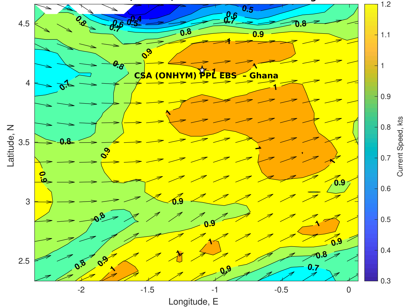
Surface Currents for CSA (ONHYM) PPL EBS - Ghana at 24-Aug-2025 00:00:00
