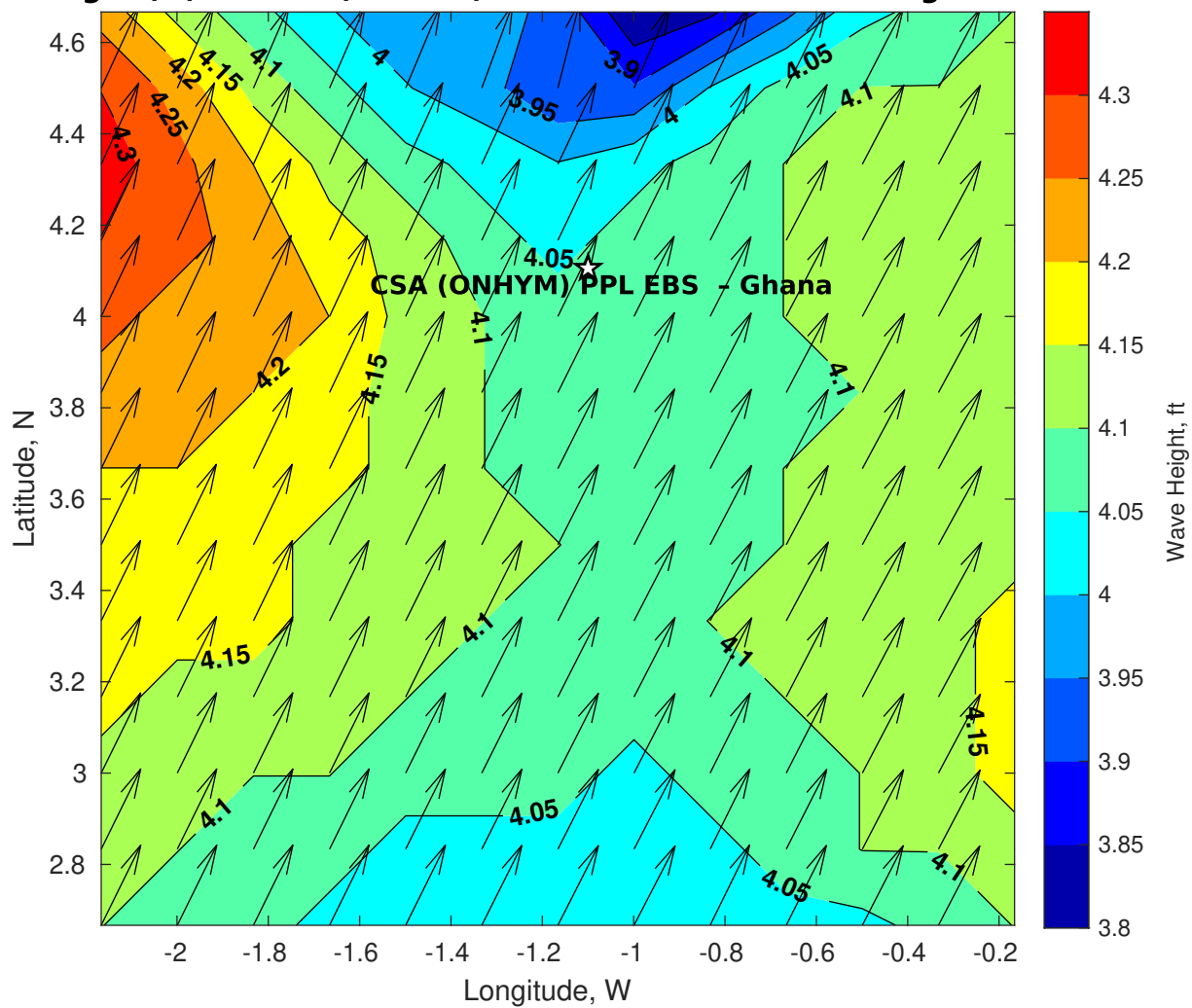
Wave Height (ft) for CSA (ONHYM) PPL EBS - Ghana at 25-Aug-2025 09:00:00
