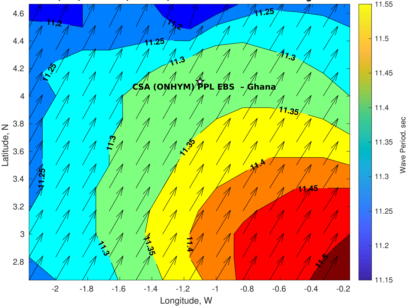
Wave Period (sec) for CSA (ONHYM) PPL EBS - Ghana at 25-Aug-2025 09:00:00
