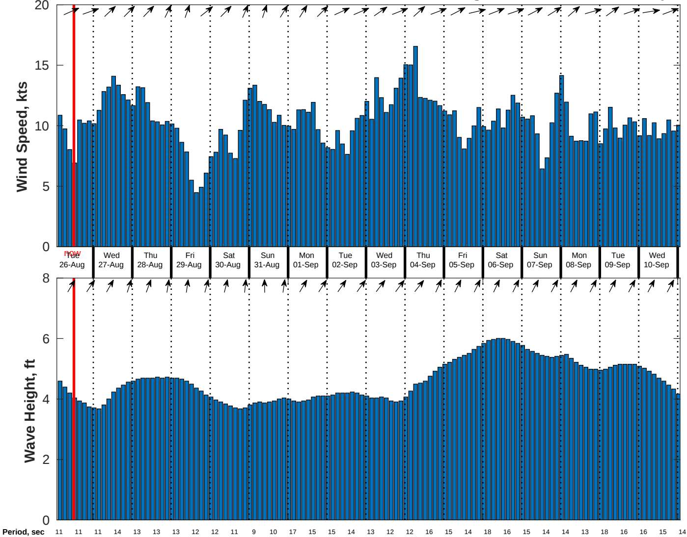
Wind & Wave Forecast for CSA (ONHYM) PPL EBS - Ghana from 25-Aug-2025 02:00:00 to 10-Sep-2025 02:00:00
