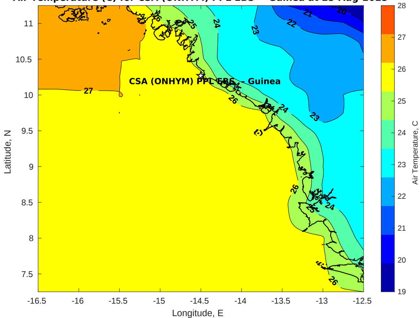
Air Temperature (C) for CSA (ONHYM) PPL EBS - Guinea at 25-Aug-2025
