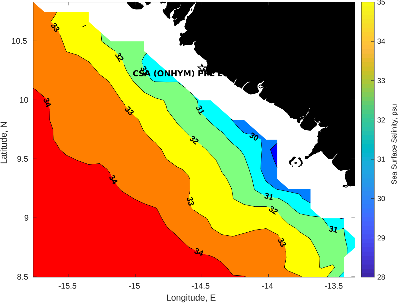
Surface Salinity for CSA (ONHYM) PPL EBS - Guinea at 24-Aug-2025 00:00:00
