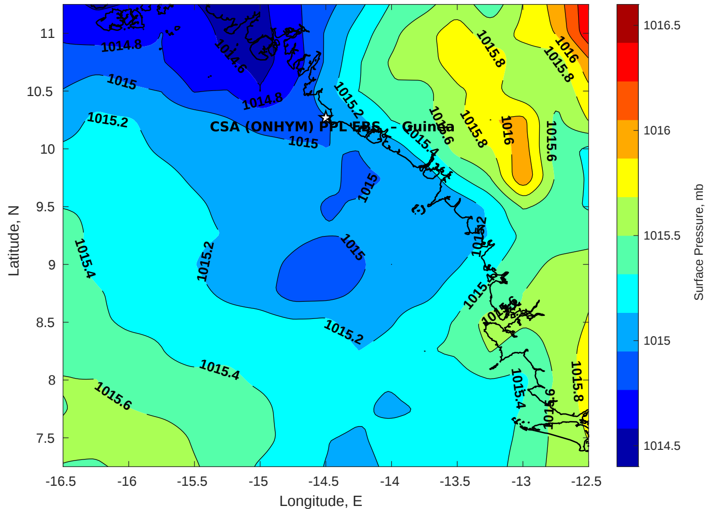
Surface Pressure (mb) for CSA (ONHYM) PPL EBS - Guinea at 25-Aug-2025 00:00:00
