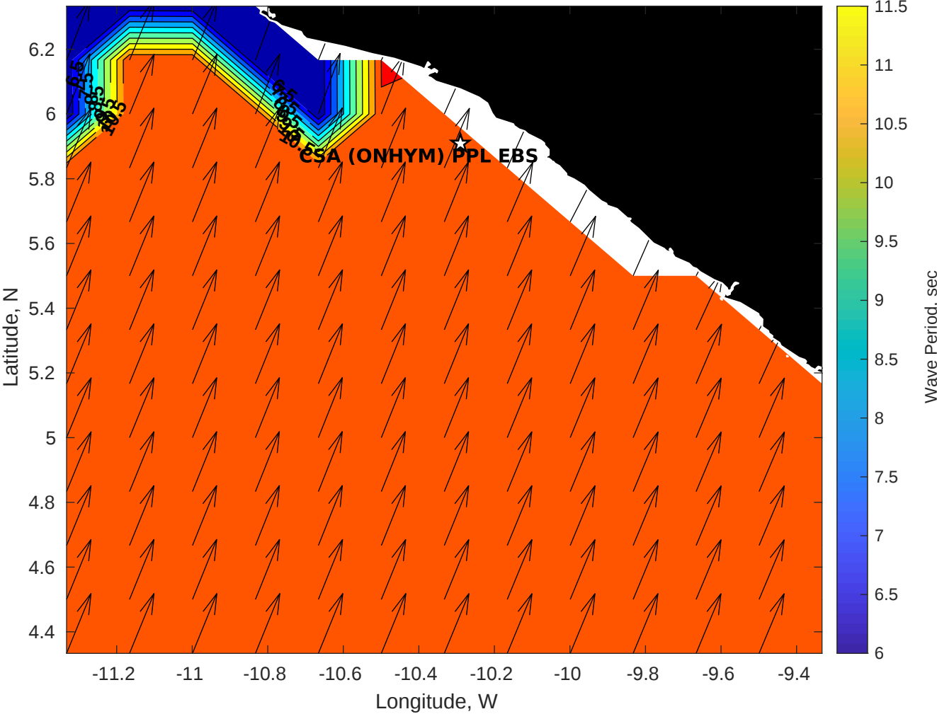
Wave Period (sec) for CSA (ONHYM) PPL EBS - Liberia at 25-Aug-2025 09:00:00
