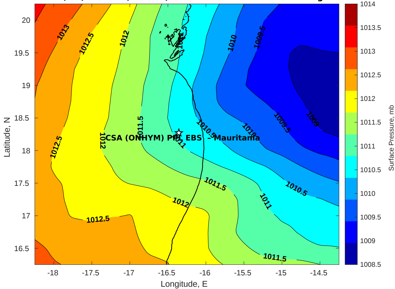
Surface Pressure (mb) for CSA (ONHYM) PPL EBS - Mauritania at 27-Aug-2025 00:00:00
