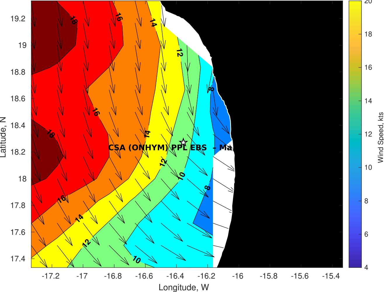
Winds (kts) for CSA (ONHYM) PPL EBS - Mauritania at 25-Aug-2025 09:00:00
