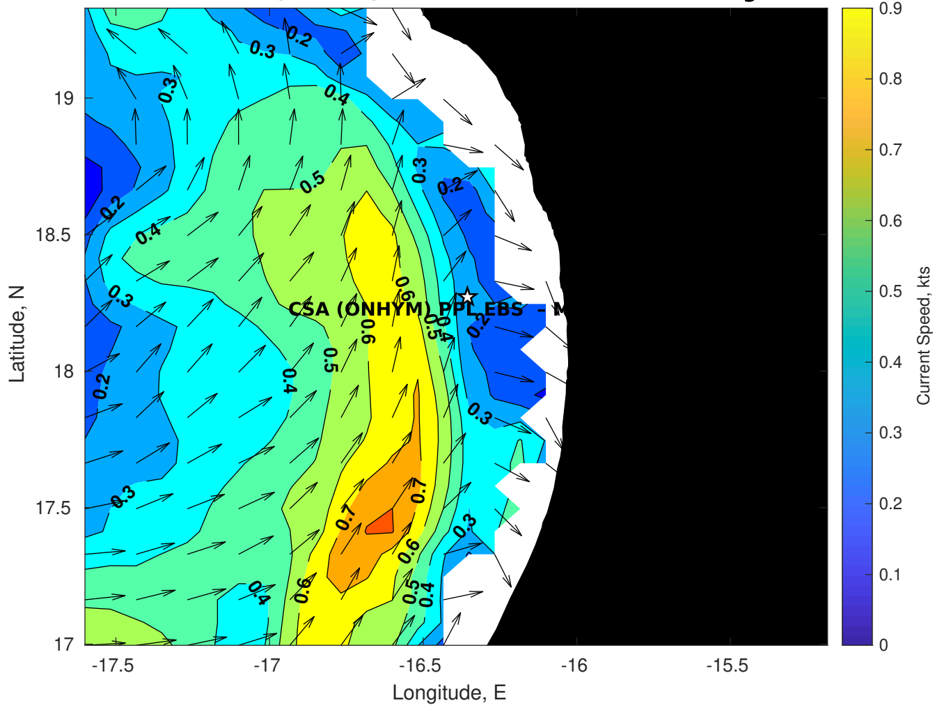
Surface Currents for CSA (ONHYM) PPL EBS - Mauritania at 24-Aug-2025 00:00:00
