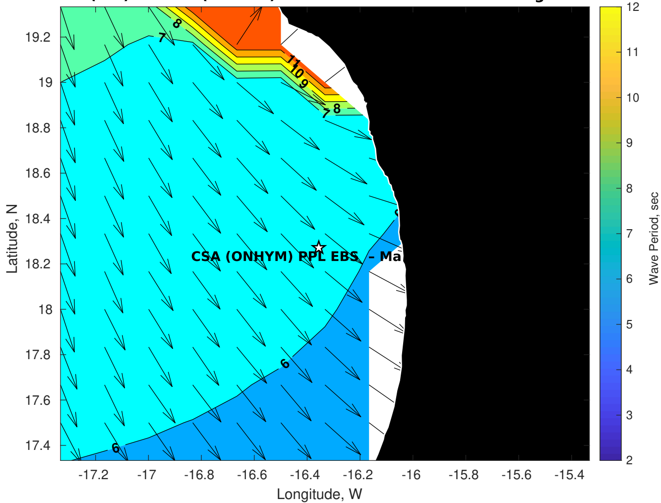
Wave Period (sec) for CSA (ONHYM) PPL EBS - Mauritania at 25-Aug-2025 09:00:00
