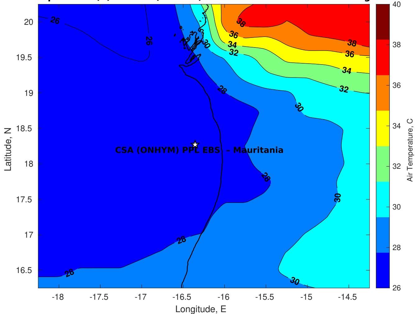
Air Temperature (C) for CSA (ONHYM) PPL EBS - Mauritania at 25-Aug-2025
