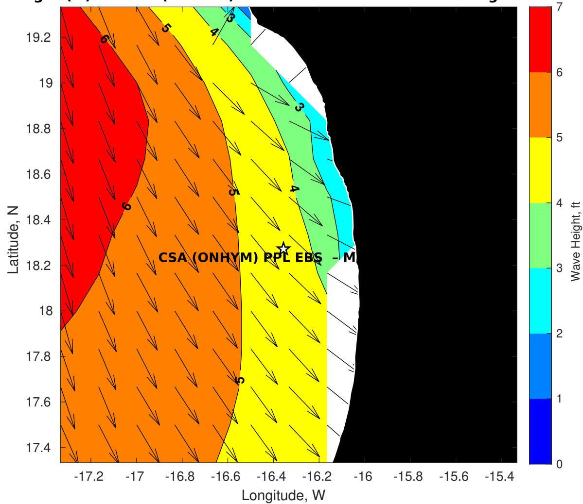
Wave Height (ft) for CSA (ONHYM) PPL EBS - Mauritania at 25-Aug-2025 09:00:00
