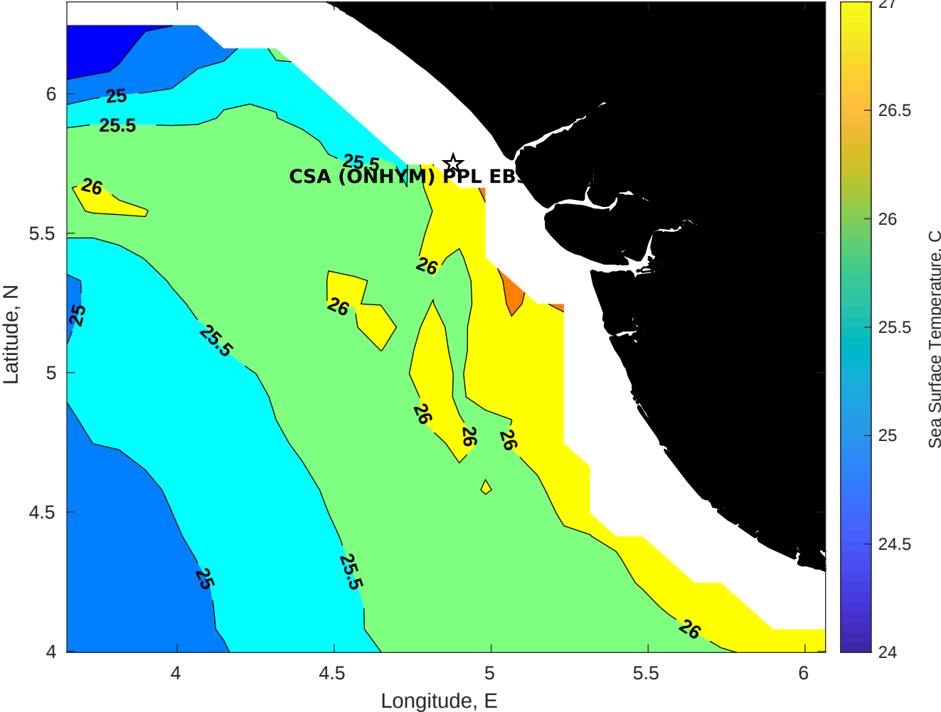
SST for CSA (ONHYM) PPL EBS - Nigeria at 24-Aug-2025 00:00:00
