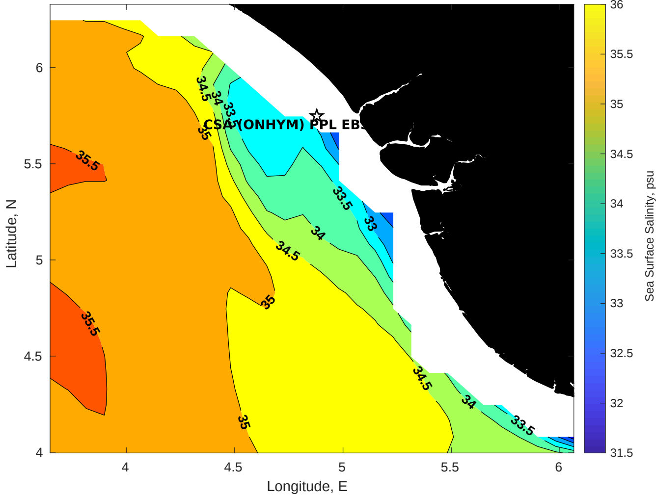
Surface Salinity for CSA (ONHYM) PPL EBS - Nigeria at 24-Aug-2025 00:00:00
