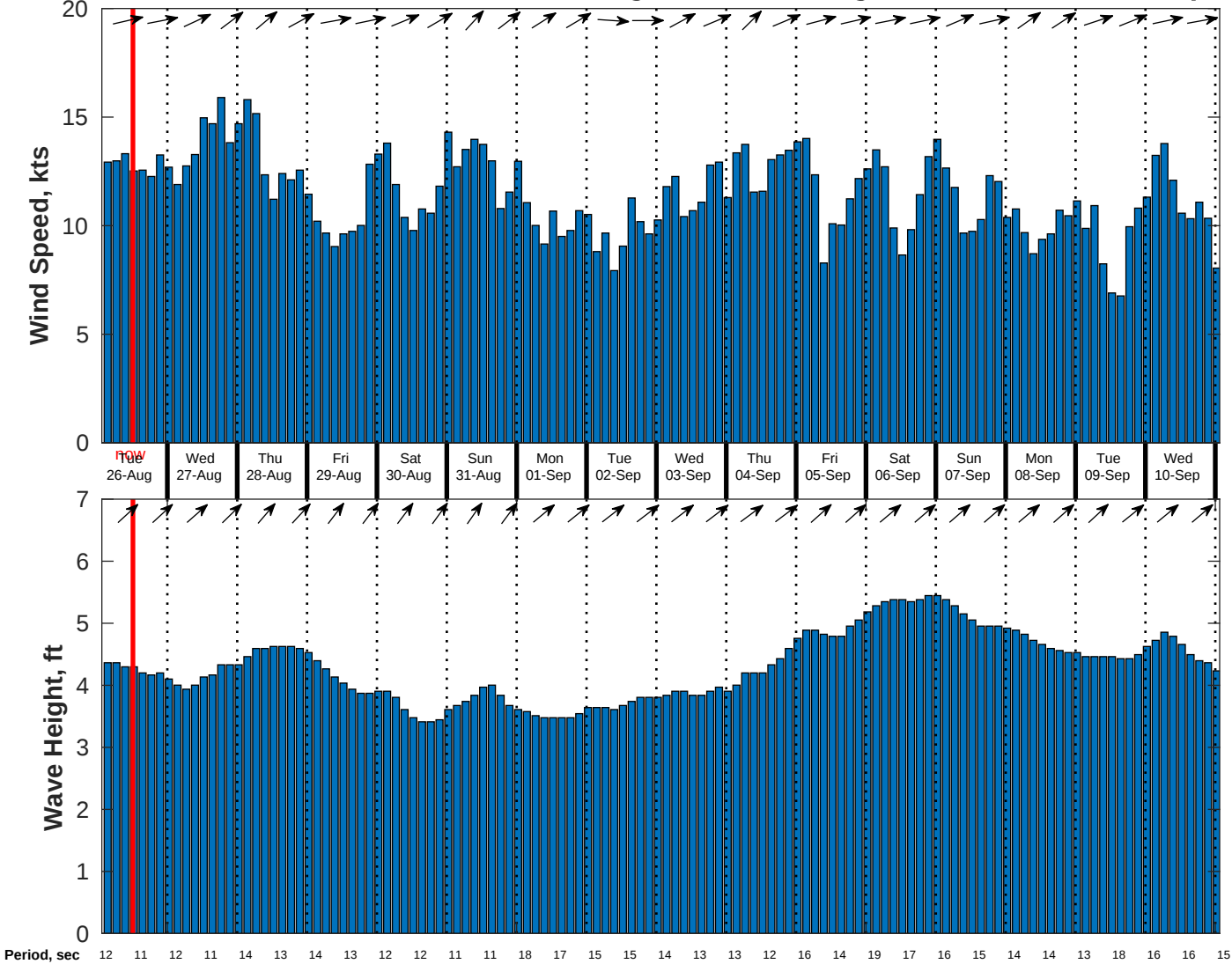
Wind & Wave Forecast for CSA (ONHYM) PPL EBS - Nigeria from 25-Aug-2025 02:00:00 to 10-Sep-2025 02:00:00
