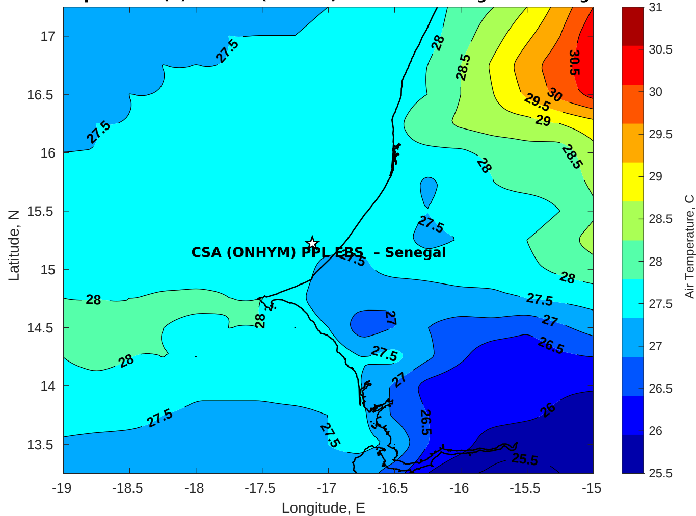
Air Temperature (C) for CSA (ONHYM) PPL EBS - Senegal at 25-Aug-2025
