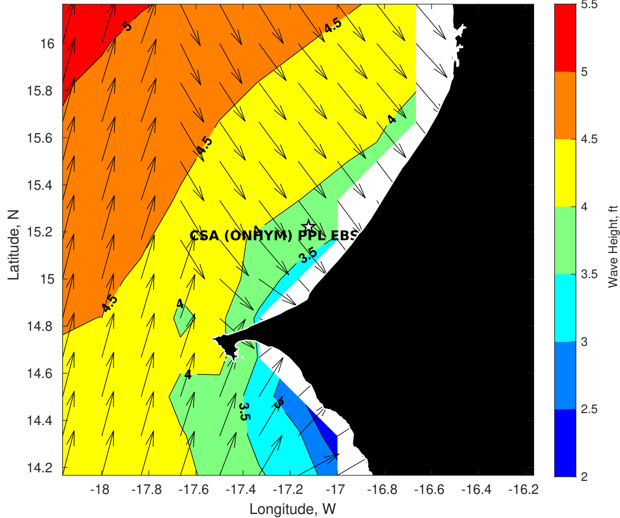
Wave Height (ft) for CSA (ONHYM) PPL EBS - Senegal at 25-Aug-2025 09:00:00
