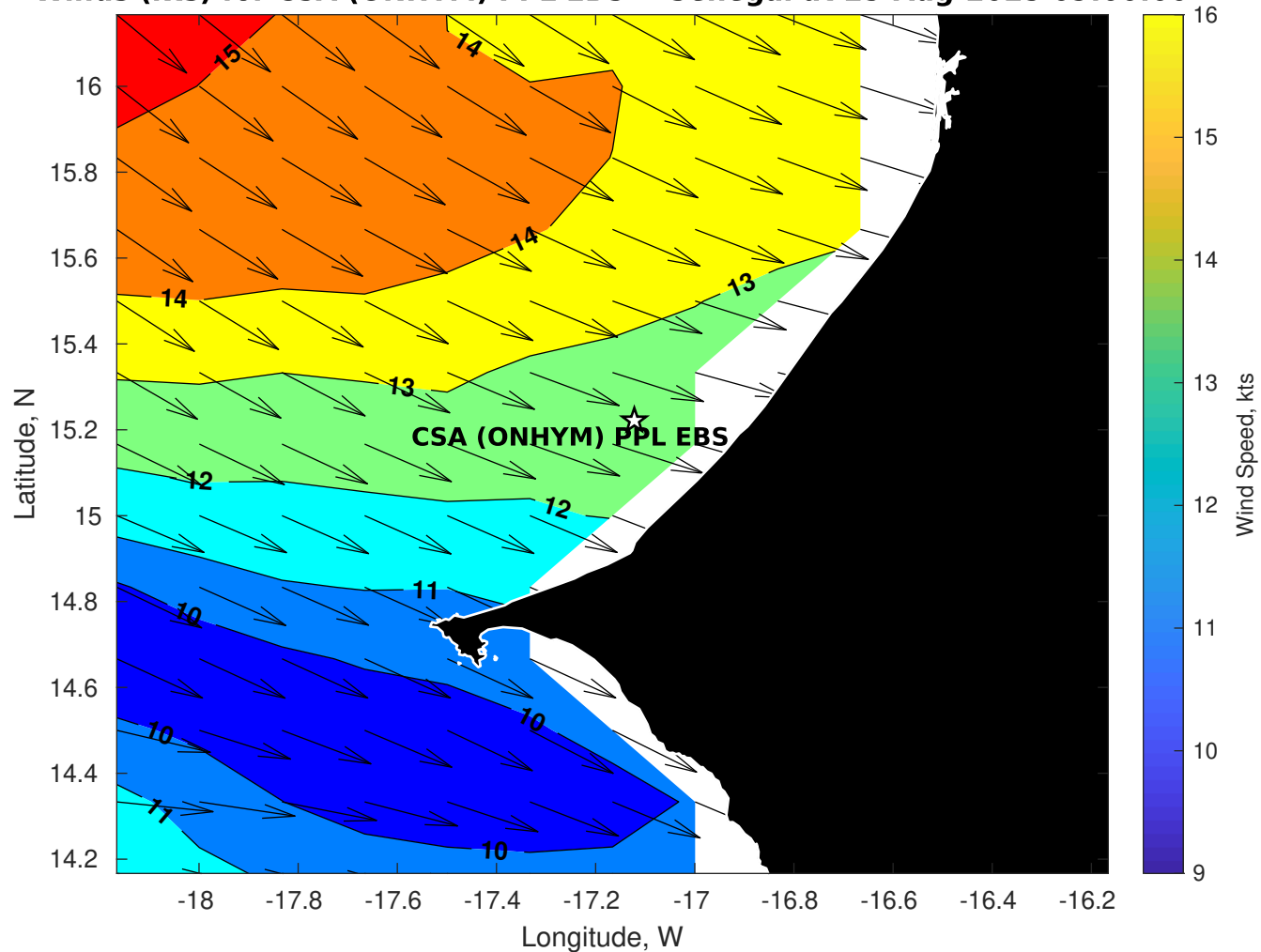
Winds (kts) for CSA (ONHYM) PPL EBS - Senegal at 25-Aug-2025 09:00:00
