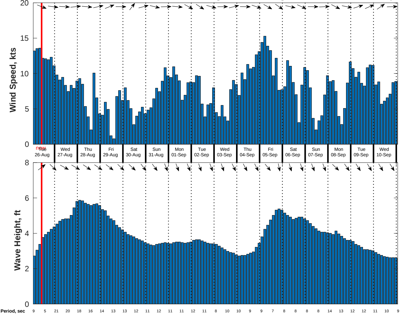
Wind & Wave Forecast for CSA (ONHYM) PPL EBS - Senegal from 25-Aug-2025 01:00:00 to 10-Sep-2025 01:00:00
