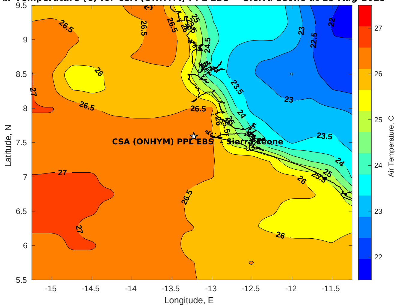
Air Temperature (C) for CSA (ONHYM) PPL EBS - Sierra Leone at 25-Aug-2025
