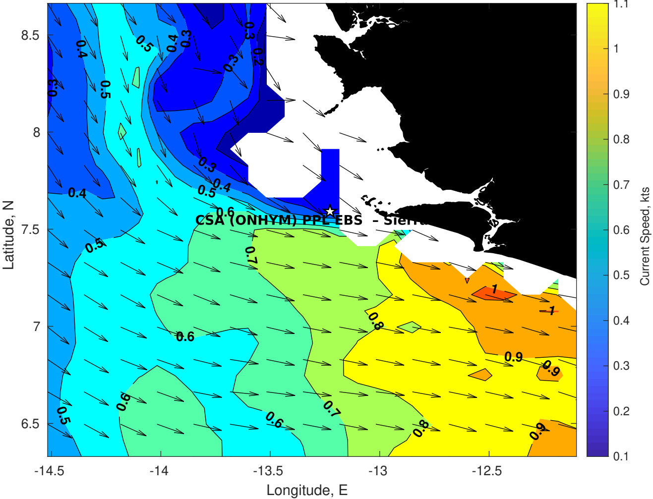
Surface Currents for CSA (ONHYM) PPL EBS - Sierra Leone at 24-Aug-2025 00:00:00
