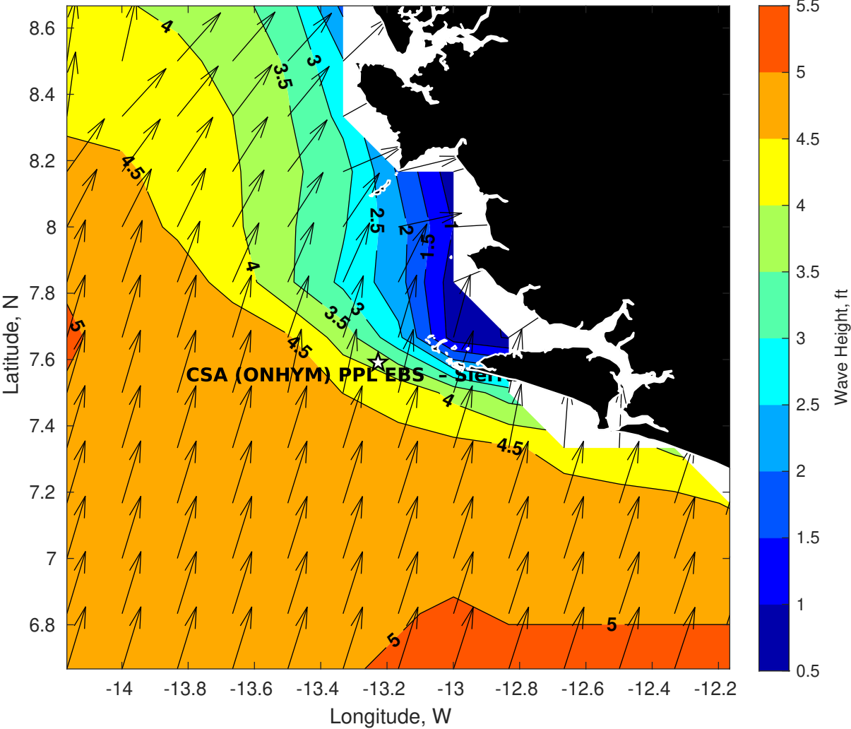
Wave Height (ft) for CSA (ONHYM) PPL EBS - Sierra Leone at 25-Aug-2025 09:00:00
