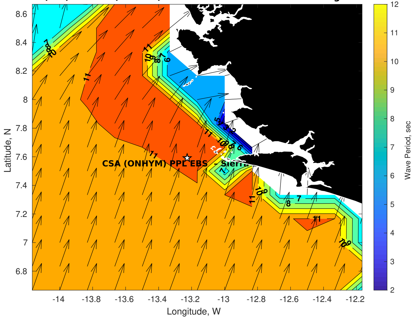
Wave Period (sec) for CSA (ONHYM) PPL EBS - Sierra Leone at 25-Aug-2025 09:00:00
