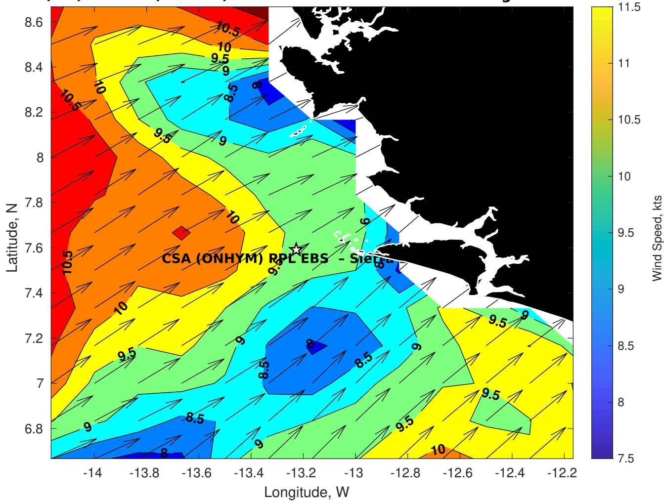
Winds (kts) for CSA (ONHYM) PPL EBS - Sierra Leone at 25-Aug-2025 09:00:00
