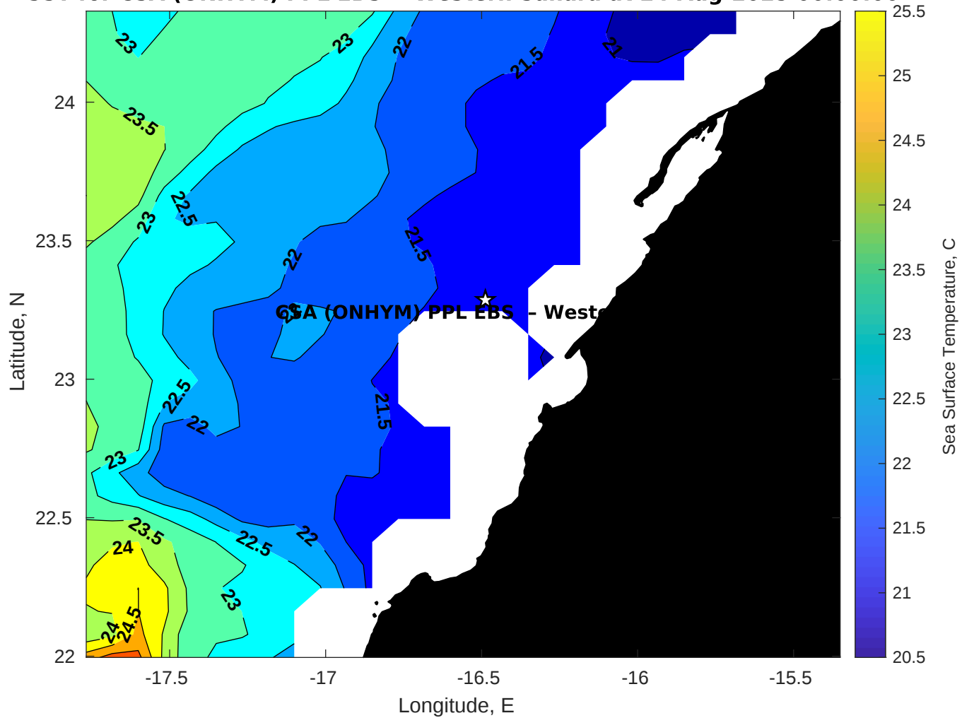
SST for CSA (ONHYM) PPL EBS - Western Sahara at 24-Aug-2025 00:00:00
