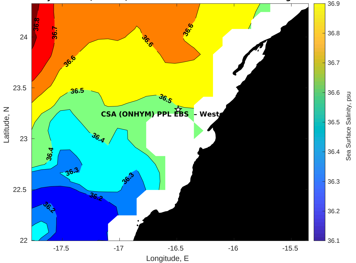
Surface Salinity for CSA (ONHYM) PPL EBS - Western Sahara at 24-Aug-2025 00:00:00
