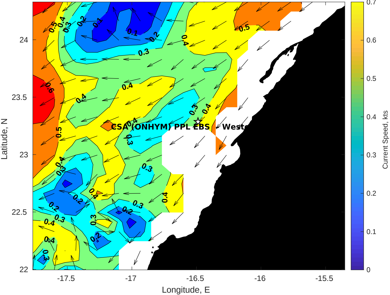
Surface Currents for CSA (ONHYM) PPL EBS - Western Sahara at 24-Aug-2025 00:00:00
