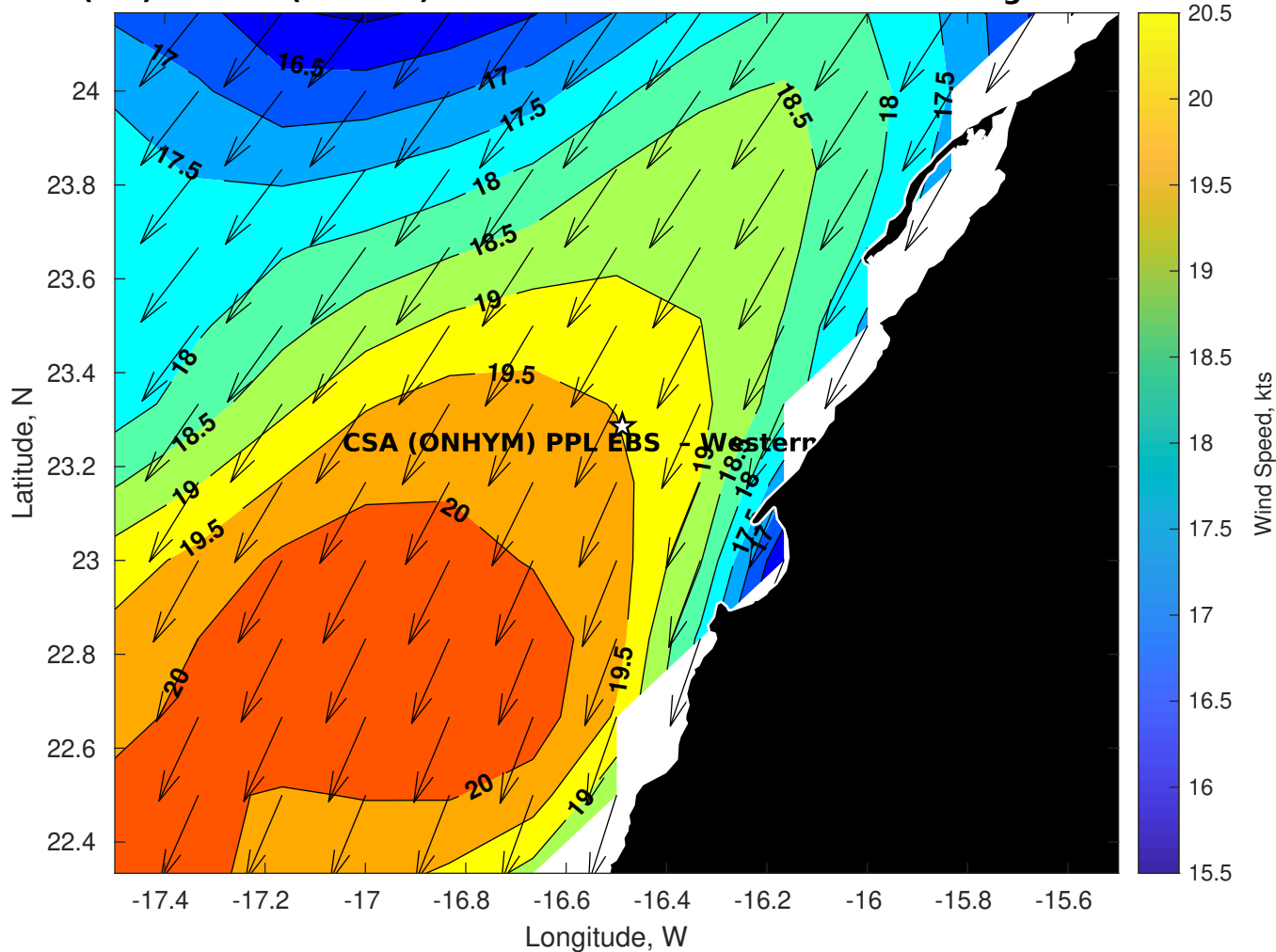
Winds (kts) for CSA (ONHYM) PPL EBS - Western Sahara at 25-Aug-2025 09:00:00
