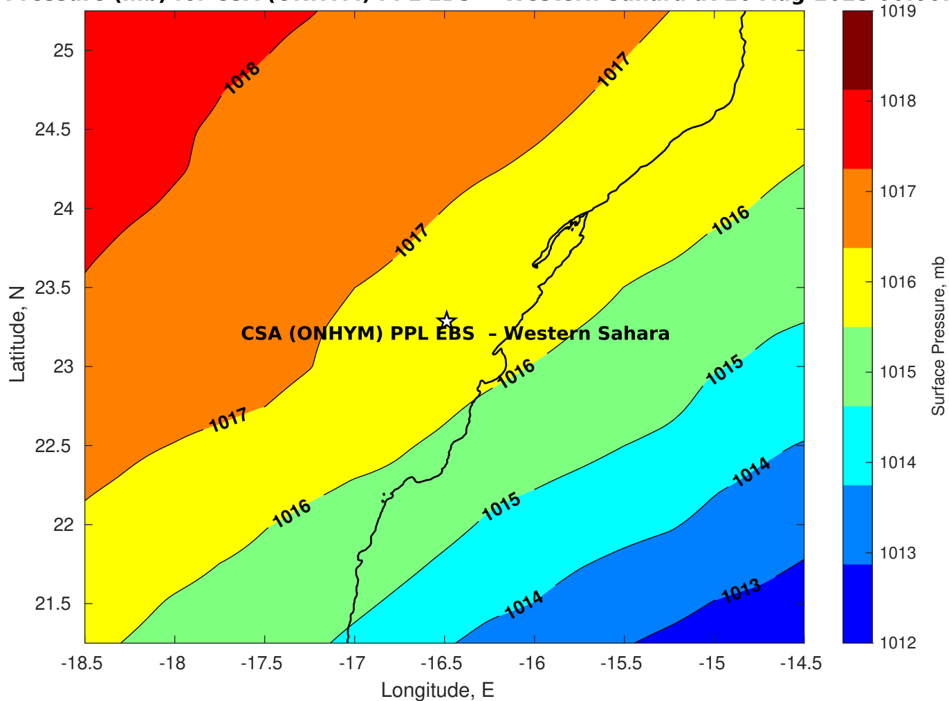
Surface Pressure (mb) for CSA (ONHYM) PPL EBS - Western Sahara at 26-Aug-2025 00:00:00
