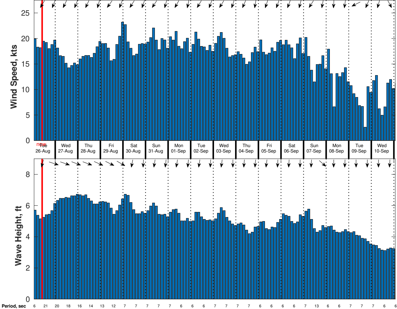
Wind & Wave Forecast for CSA (ONHYM) PPL EBS - Western Sahara from 25-Aug-2025 01:00:00 to 10-Sep-2025 01:00:00
