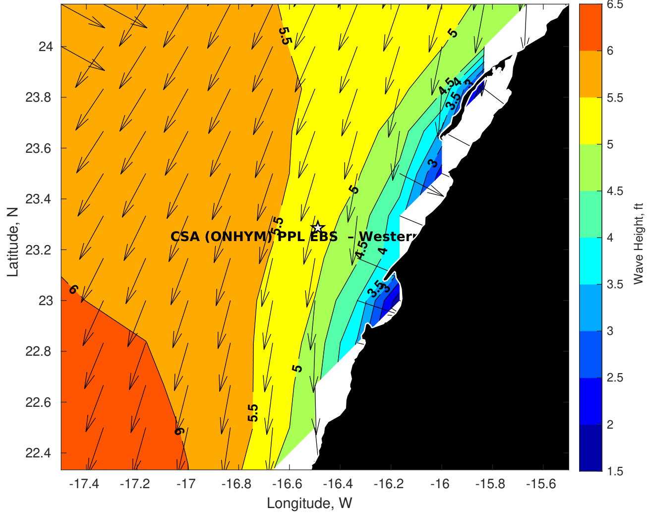
Wave Height (ft) for CSA (ONHYM) PPL EBS - Western Sahara at 25-Aug-2025 09:00:00
