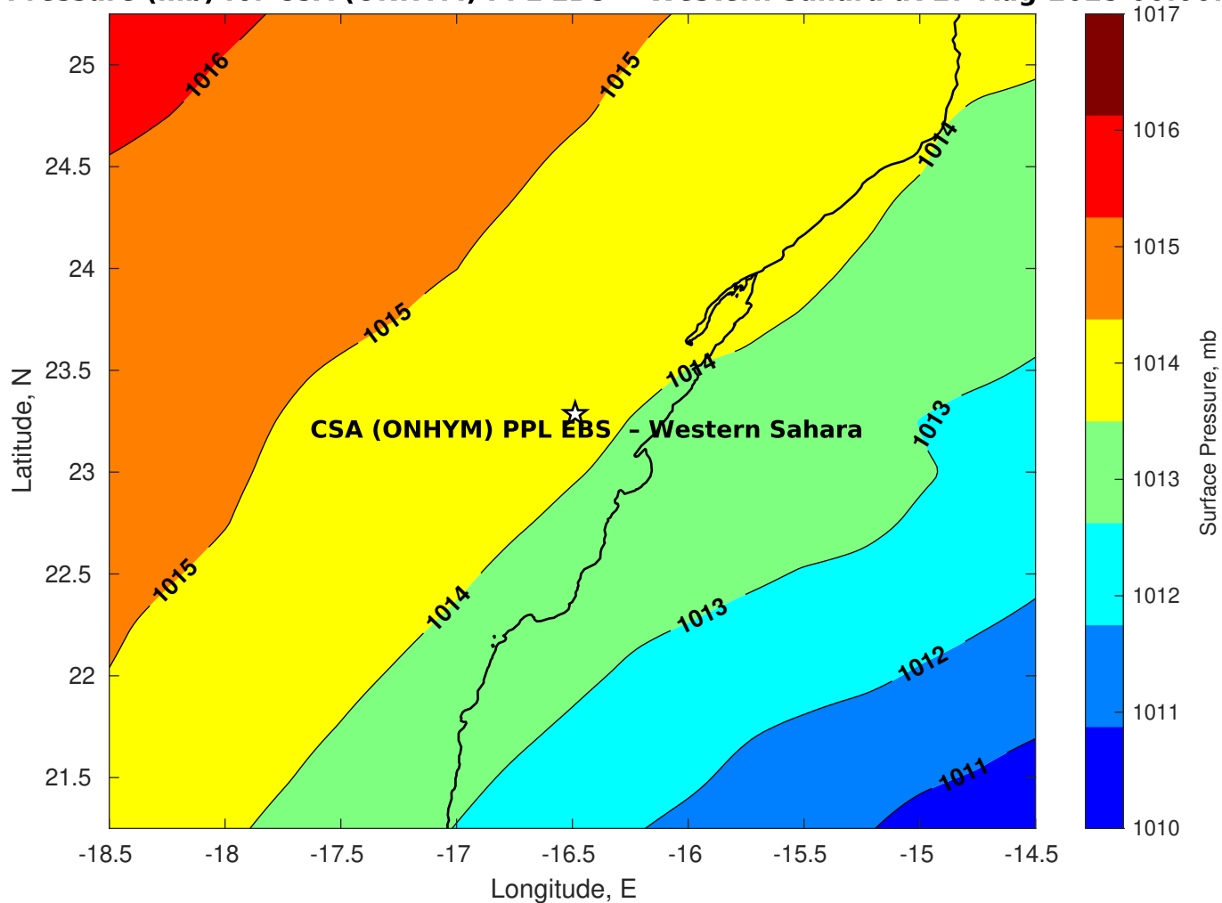
Surface Pressure (mb) for CSA (ONHYM) PPL EBS - Western Sahara at 27-Aug-2025 00:00:00
