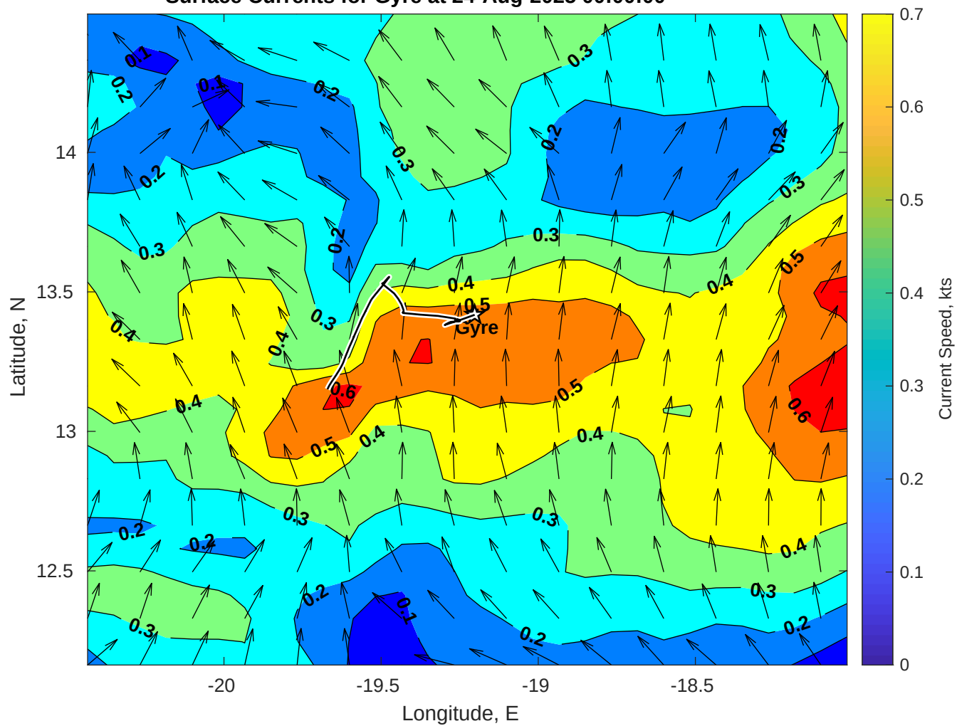
Surface Currents for Gyre at 24-Aug-2025 00:00:00
