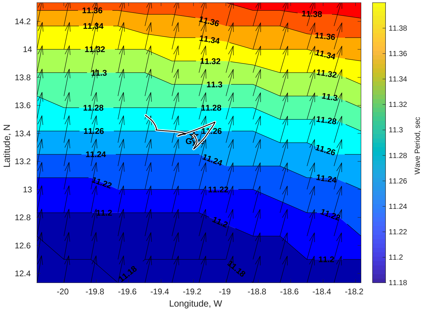
Wave Period (sec) for Gyre at 25-Aug-2025 09:00:00
