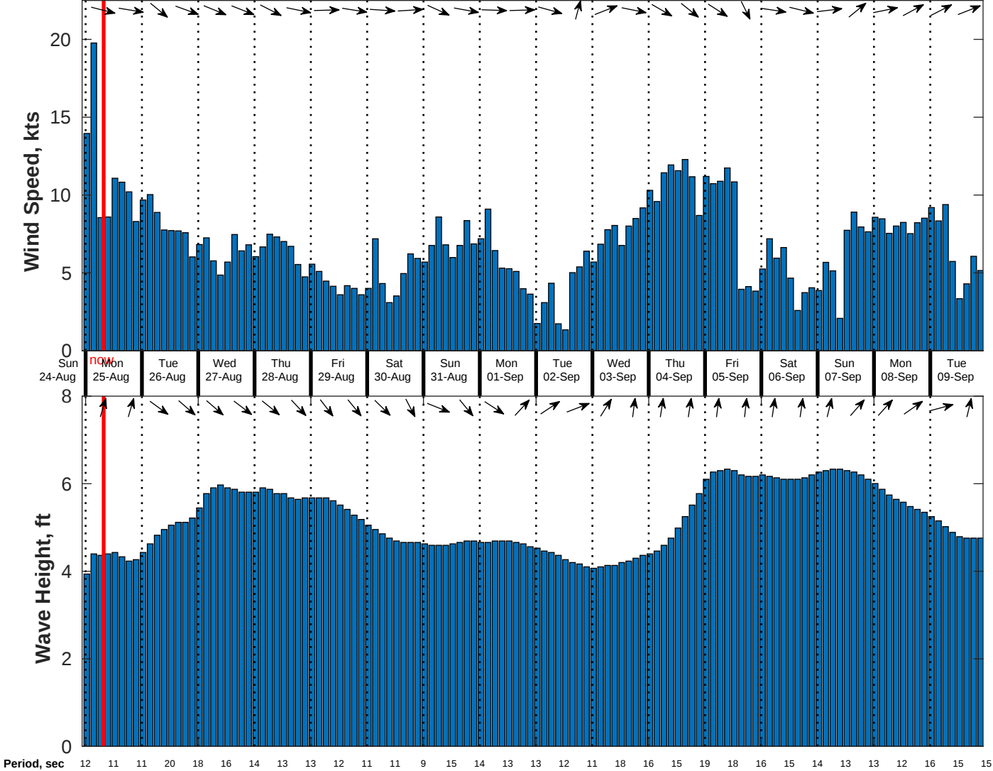
Wind & Wave Forecast for Gyre from 24-Aug-2025 23:00:00 to 09-Sep-2025 23:00:00
