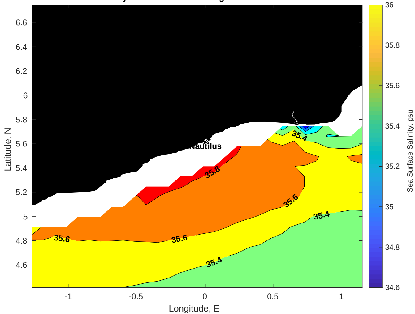
Surface Salinity for Nautilus at 24-Aug-2025 00:00:00
