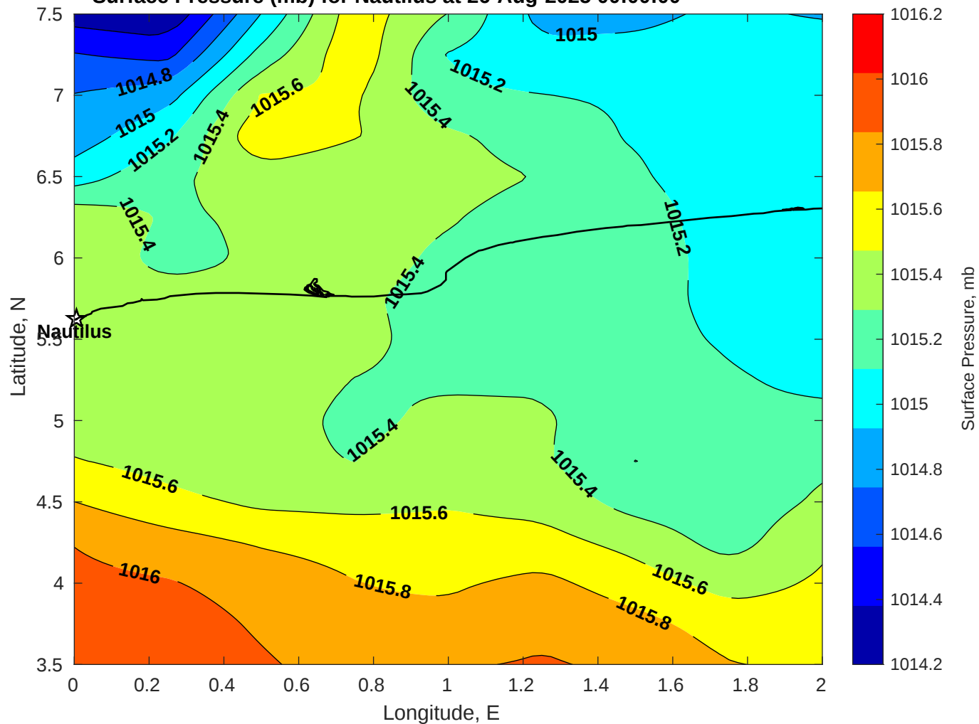
Surface Pressure (mb) for Nautilus at 26-Aug-2025 00:00:00
