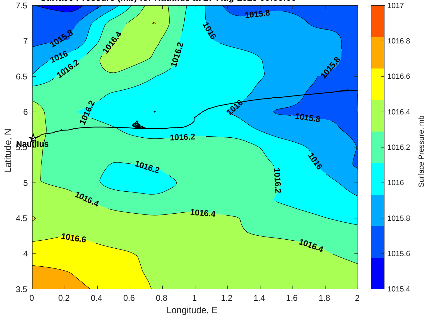
Surface Pressure (mb) for Nautilus at 27-Aug-2025 00:00:00
