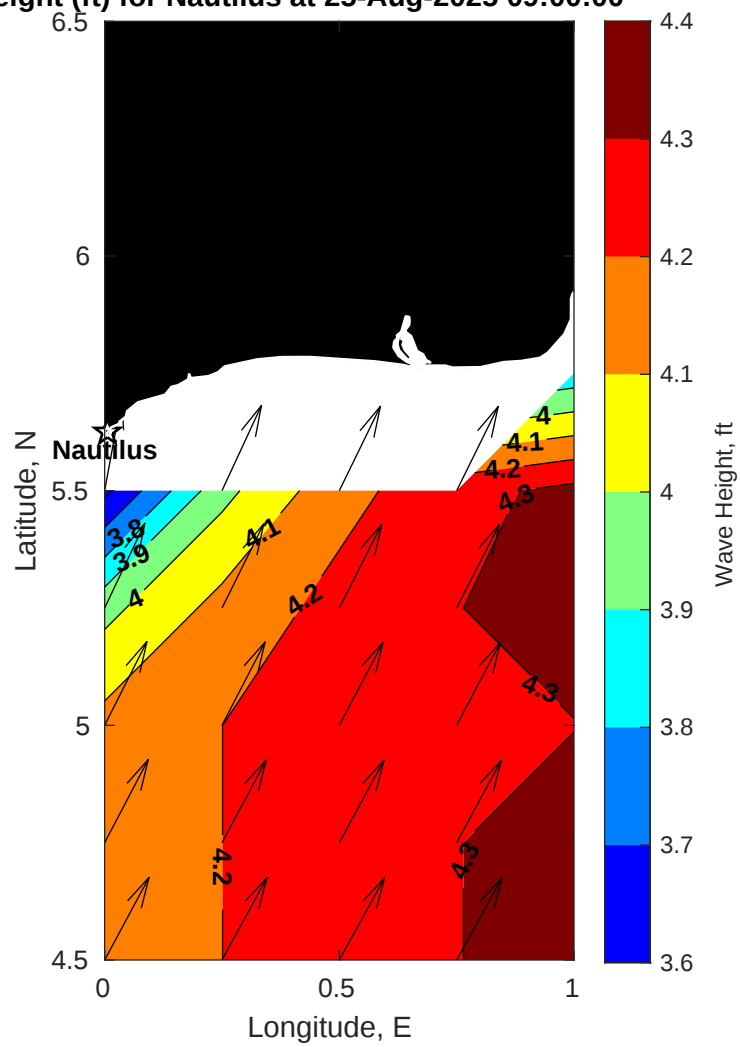
Wave Height (ft) for Nautilus at 25-Aug-2025 09:00:00
