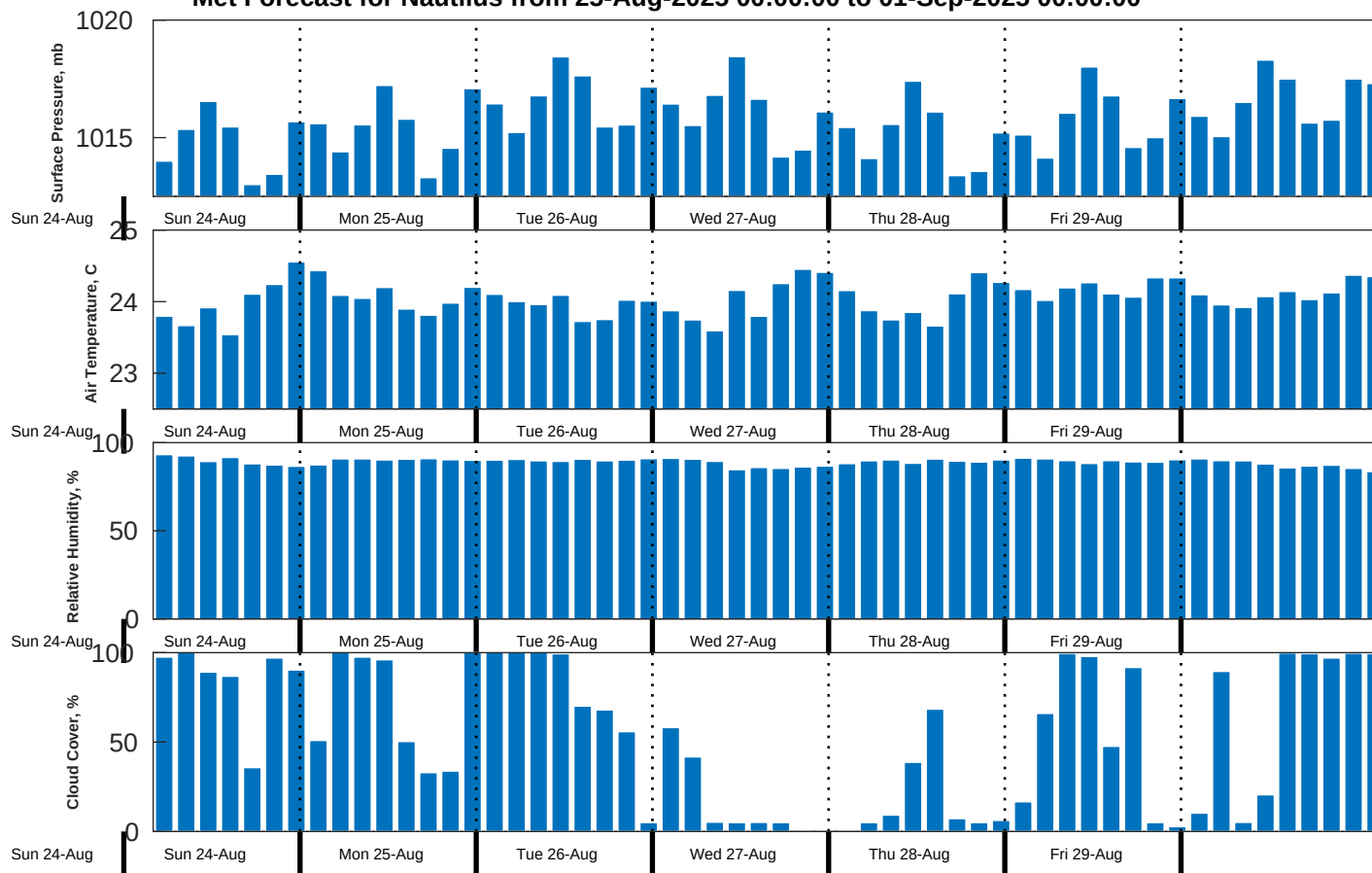
Met Forecast for Nautilus from 25-Aug-2025 00:00:00 to 01-Sep-2025 00:00:00
